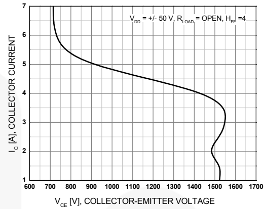
Figure 17. BJT RBSOA
