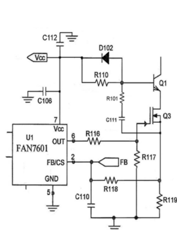
Figure 31. V_{CC} Derived
