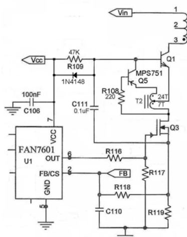
Figure 33. Proportional Drive
