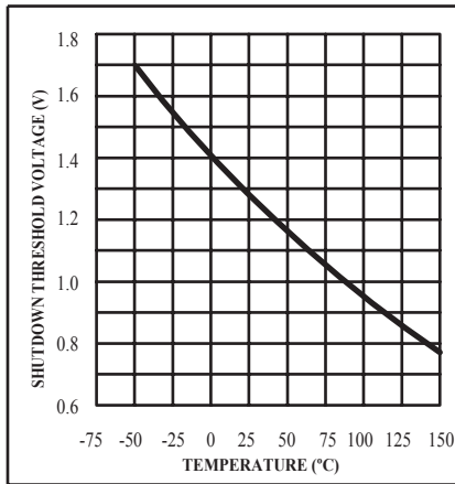
Shutdown Threshold Voltage
