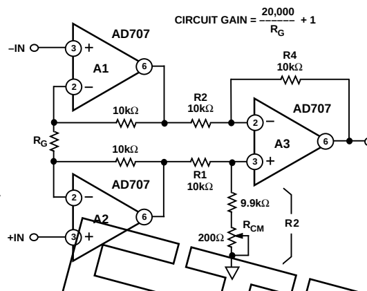
Figure 24. A 3 Op Amp Instrumentation Amplifier
