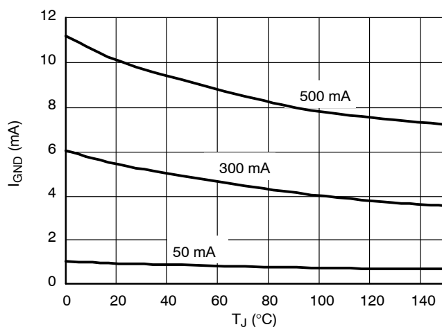
Figure 3. Ground Current vs. Temperature
