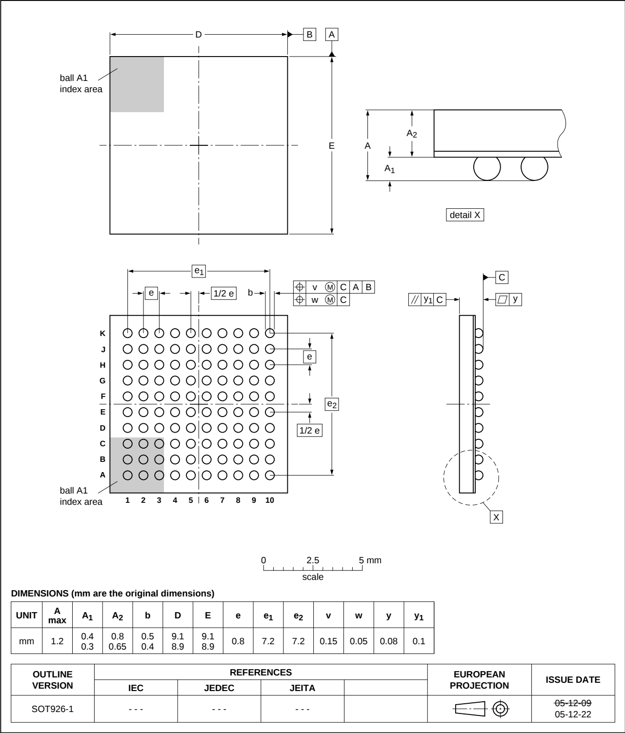
Fig 54. TFBGA100 package
