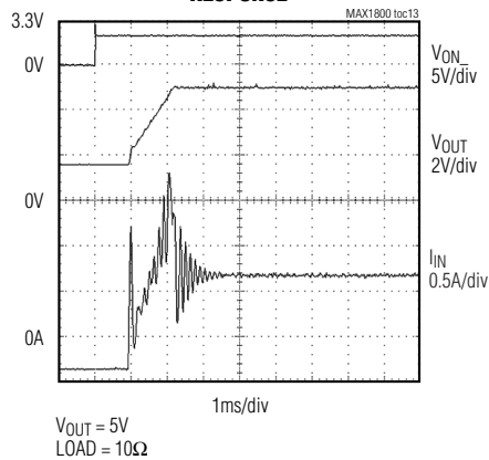
AUXILIARY CONTROLLER STARTUP RESPONSE
