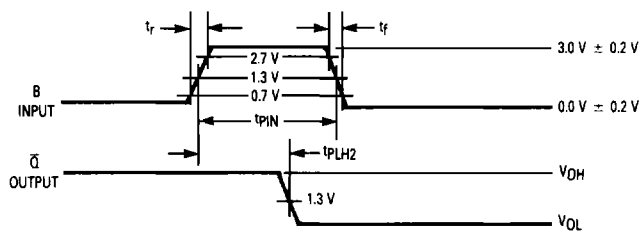
tPHL2 Waveforms
