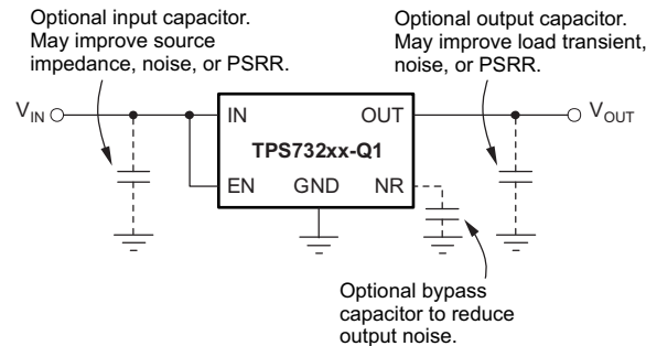
Figure 29. Typical Application Circuit for Fixed-Voltage Versions
