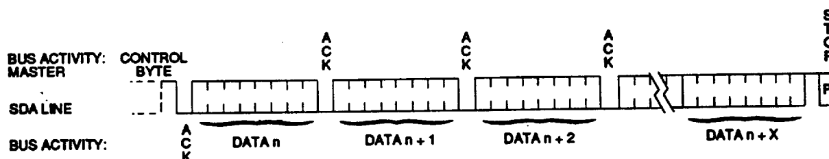
FIGURE 7 - SEQUENTIAL READ
