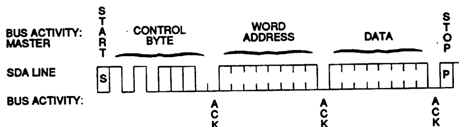
FIGURE 3 - BYTE WRITE
