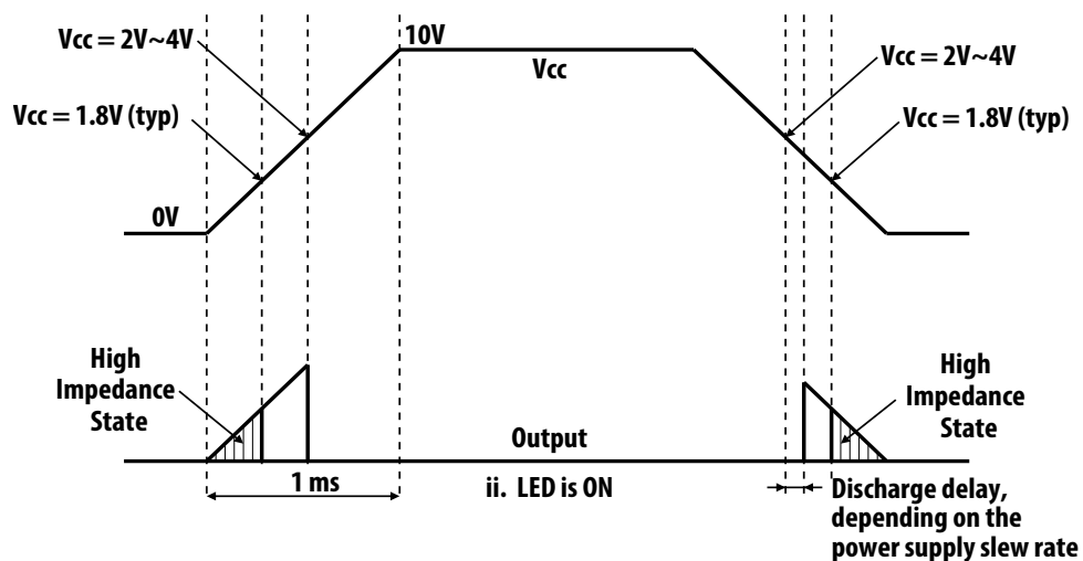
Figure 11: V_{CC} Ramp When LED Is OFF
