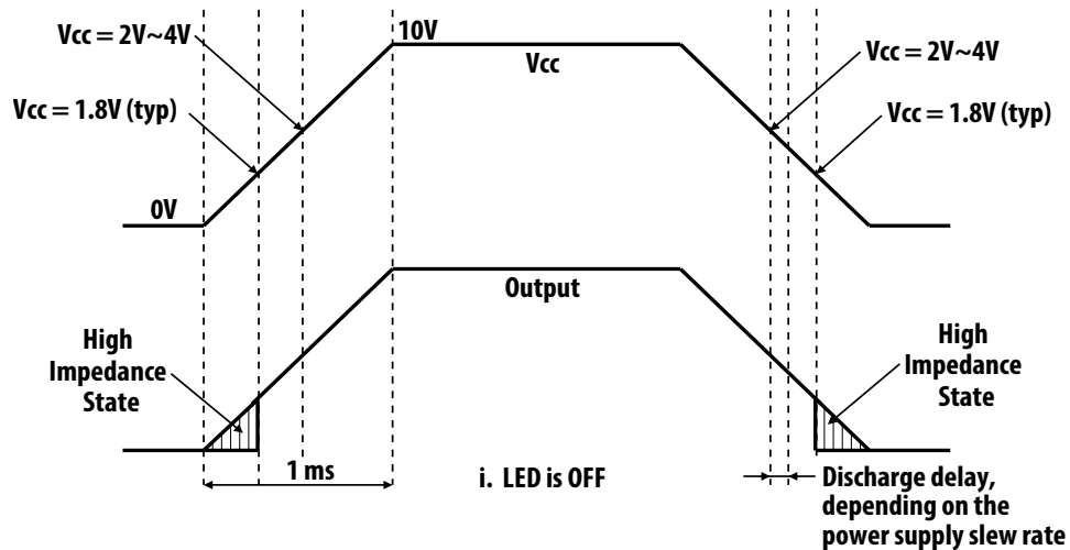
Figure 10: V_{CC} Ramp When LED Is ON
