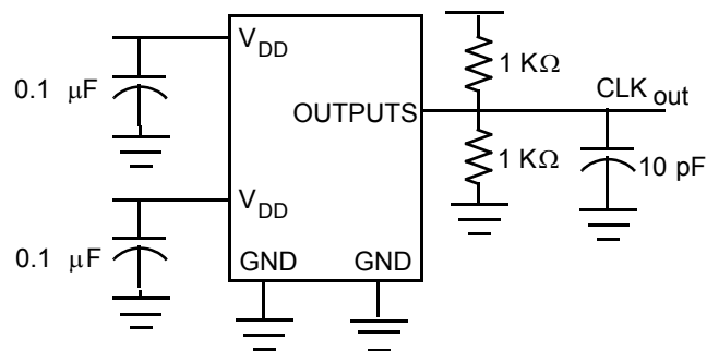
Test Circuit # 2
