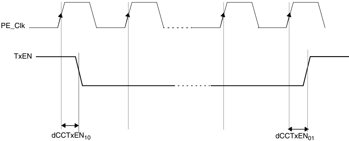
Figure 19. FlexRay TxEN signal propagation delays
