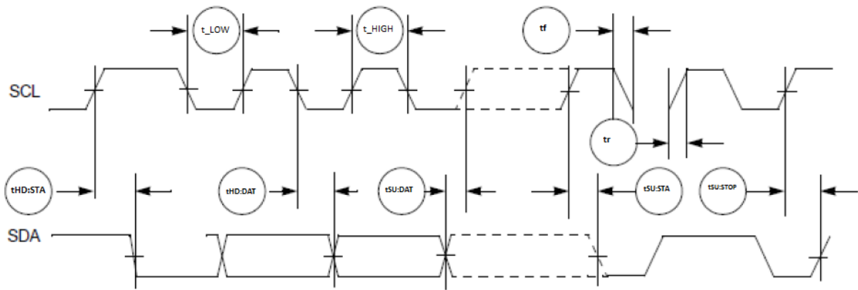
Figure 32. I²C input/output timing
