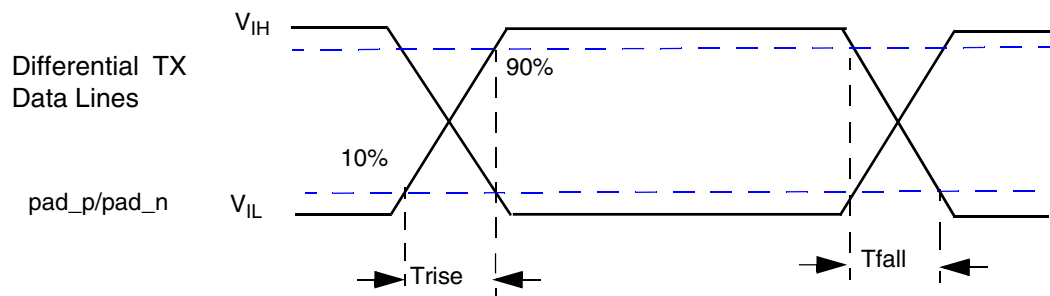
Figure 24. Rise/fall time
