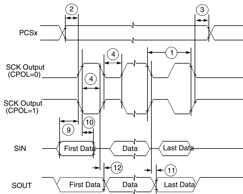
Figure 25. SPI classic SPI timing — master, CPHA = 0
