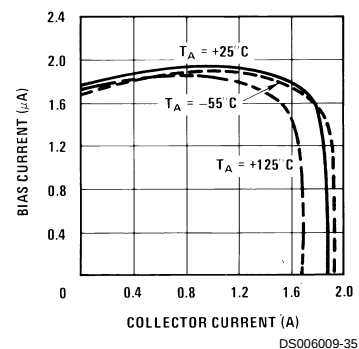
Bias Current
