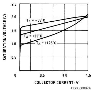
Saturation Voltage
