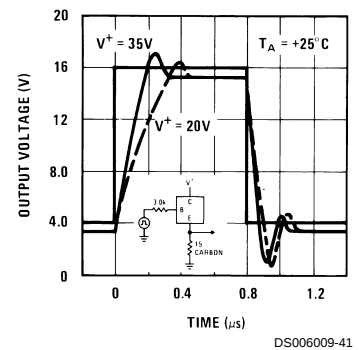
Response Time
