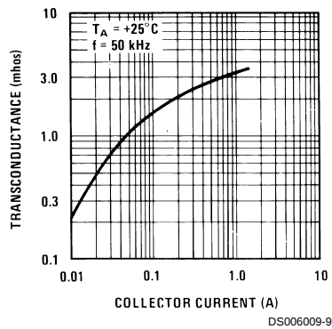
Transconductance
