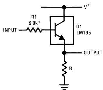
Emitter Follower
