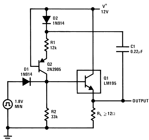
Power One-Shot
