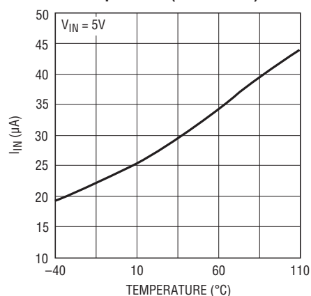
Burst Mode Current vs Temperature (LTC1983-3)
