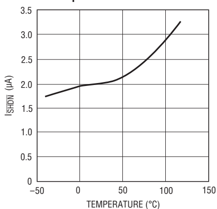
\overline{\text{SHDN}} Pin Input Current vs Temperature
