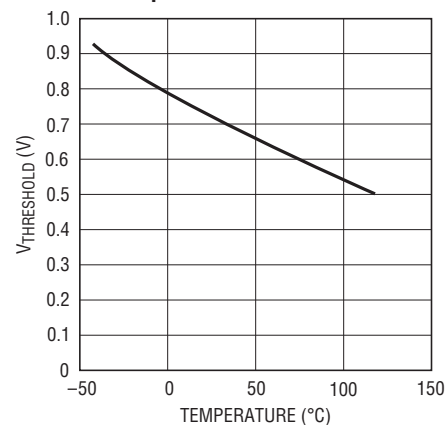
\overline{\text{SHDN}} Pin Threshold Voltage vs Temperature
