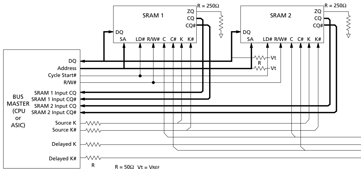
Figure 3: Application Example
