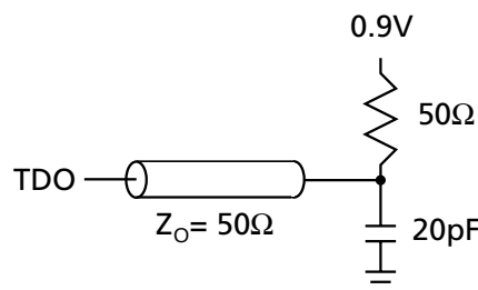
Figure 10: TAP AC Output Load Equivalent
