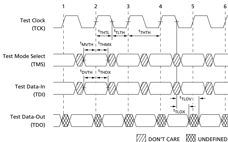
Figure 9: TAP Timing
