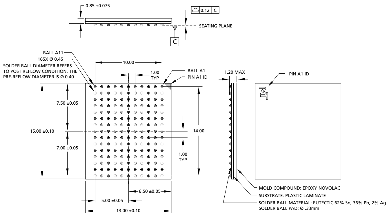
Figure 11: 165-Ball FBGA
