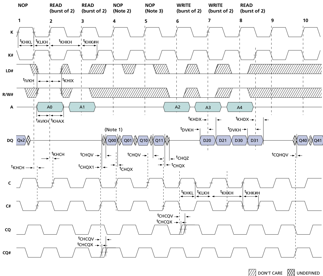
Figure 6: READ/WRITE Timing
