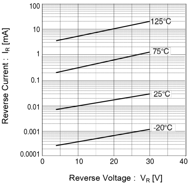
Fig.12 Reverse Current vs. Reverse Voltage
