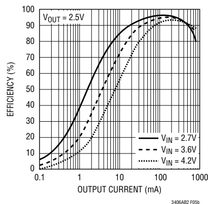
Figure 5b. Efficiency vs Load Current
