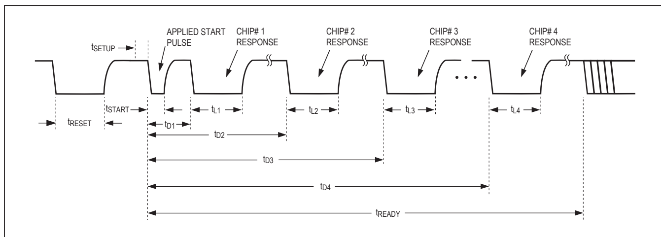
Figure 1. Timing Diagram
