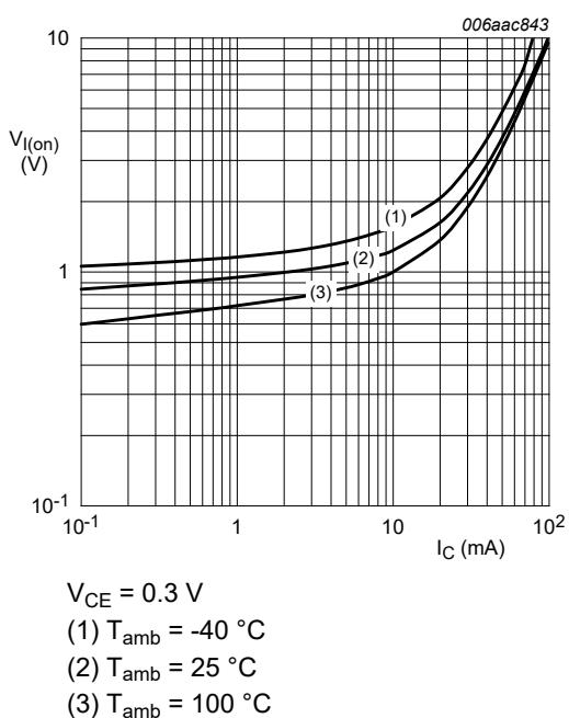
Fig. 7. PDTC143XQC: On-state input voltage as a function of collector current; typical values
