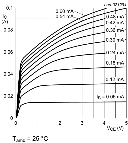
Fig. 29. PDTC124XQC: Collector current as a function of collector-emitter voltage; typical values
