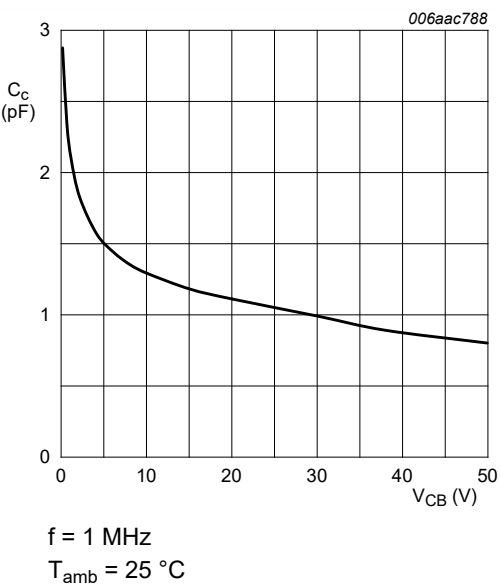
Fig. 27. PDTC114YQC: Collector capacitance as a function of collector-base voltage; typical values
