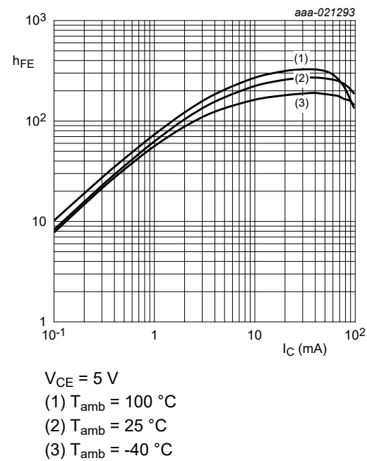
Fig. 28. PDTC124XQC: DC current gain as a function of collector current; typical values
