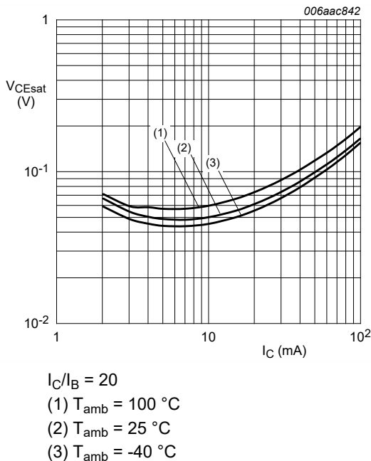
Fig. 6. PDTC143XQC: Collector-emitter saturation voltage as a function of collector current; typical values
