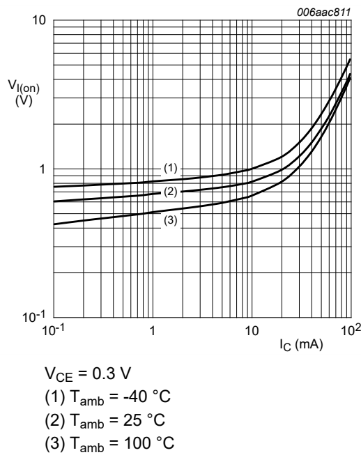
Fig. 13. PDTC123JQC: On-state input voltage as a function of collector current; typical values
