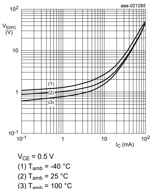
Fig. 31. PDTC124XQC: On-state input voltage as a function of collector current; typical values
