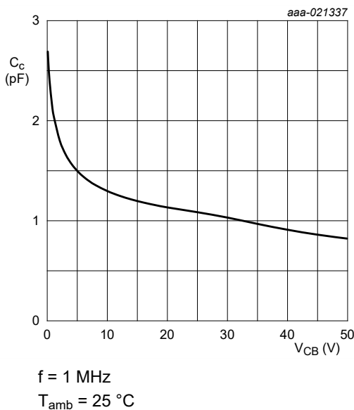
Fig. 33. PDTC124XQC: Collector capacitance as a function of collector-base voltage; typical values
