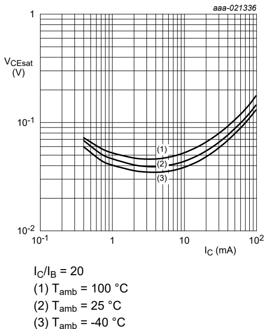
Fig. 30. PDTC124XQC: Collector-emitter saturation voltage as a function of collector current; typical values
