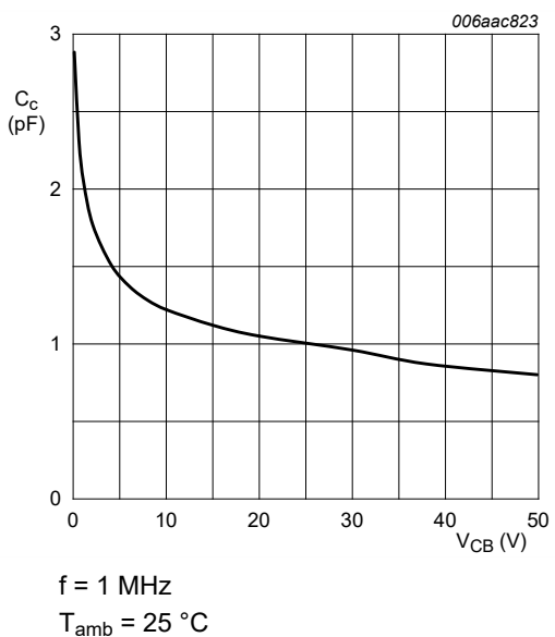
Fig. 21. PDTC143ZQC: Collector capacitance as a function of collector-base voltage; typical values
