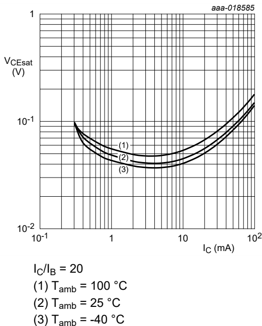
Fig. 18. PDTC143ZQC: Collector-emitter saturation voltage as a function of collector current; typical values
