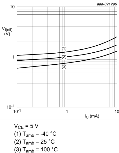
Fig. 32. PDTC124XQC: Off-state input voltage as a function of collector current; typical values
