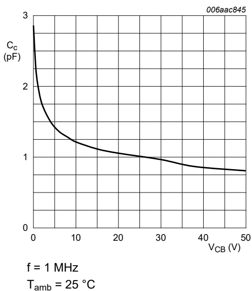
Fig. 9. PDTC143XQC: Collector capacitance as a function of collector-base voltage; typical values
