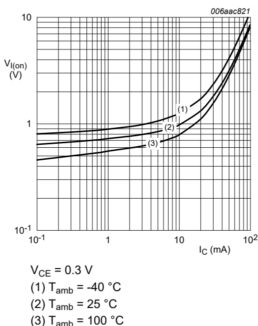
Fig. 19. PDTC143ZQC: On-state input voltage as a function of collector current; typical values
