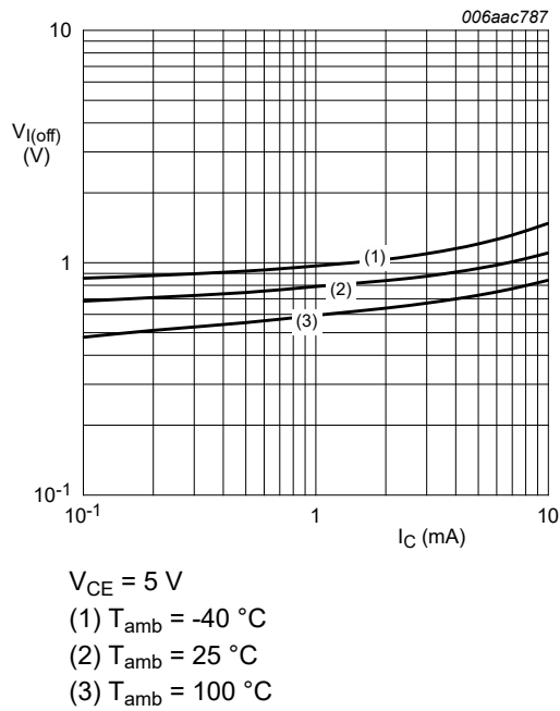
Fig. 26. PDTC114YQC: Off-state input voltage as a function of collector current; typical values
