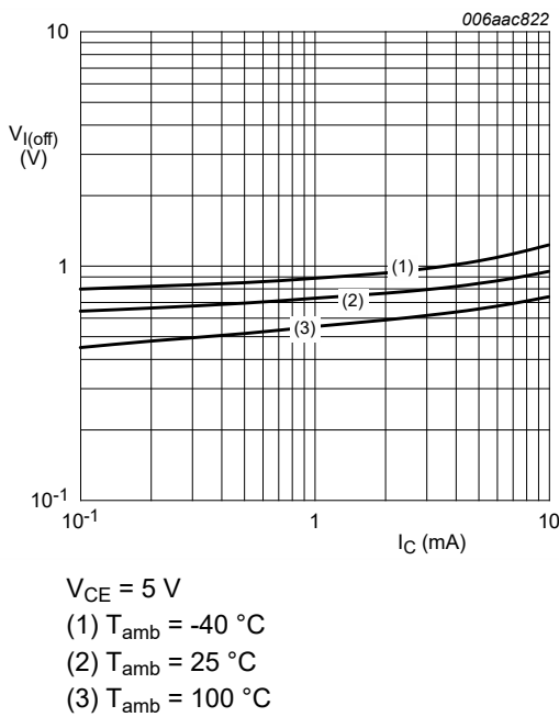
Fig. 20. PDTC143ZQC: Off-state input voltage as a function of collector current; typical values
