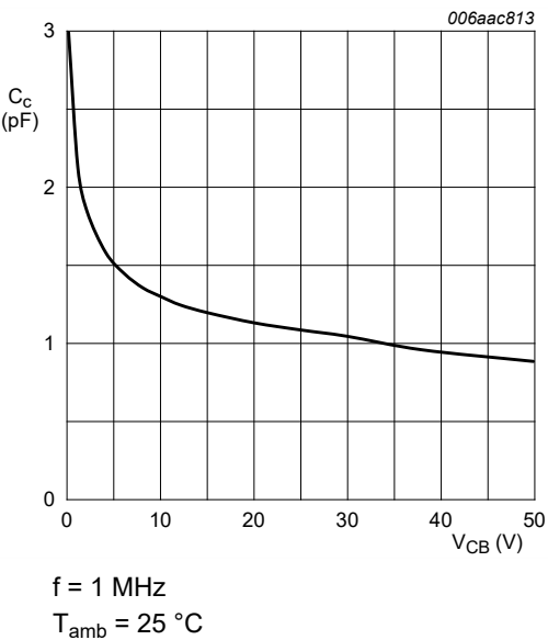
Fig. 15. PDTC123JQC: Collector capacitance as a function of collector-base voltage; typical values
