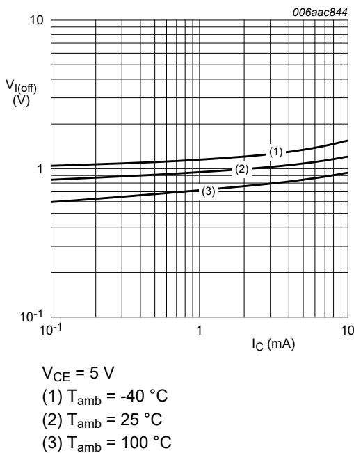
Fig. 8. PDTC143XQC: Off-state input voltage as a function of collector current; typical values
