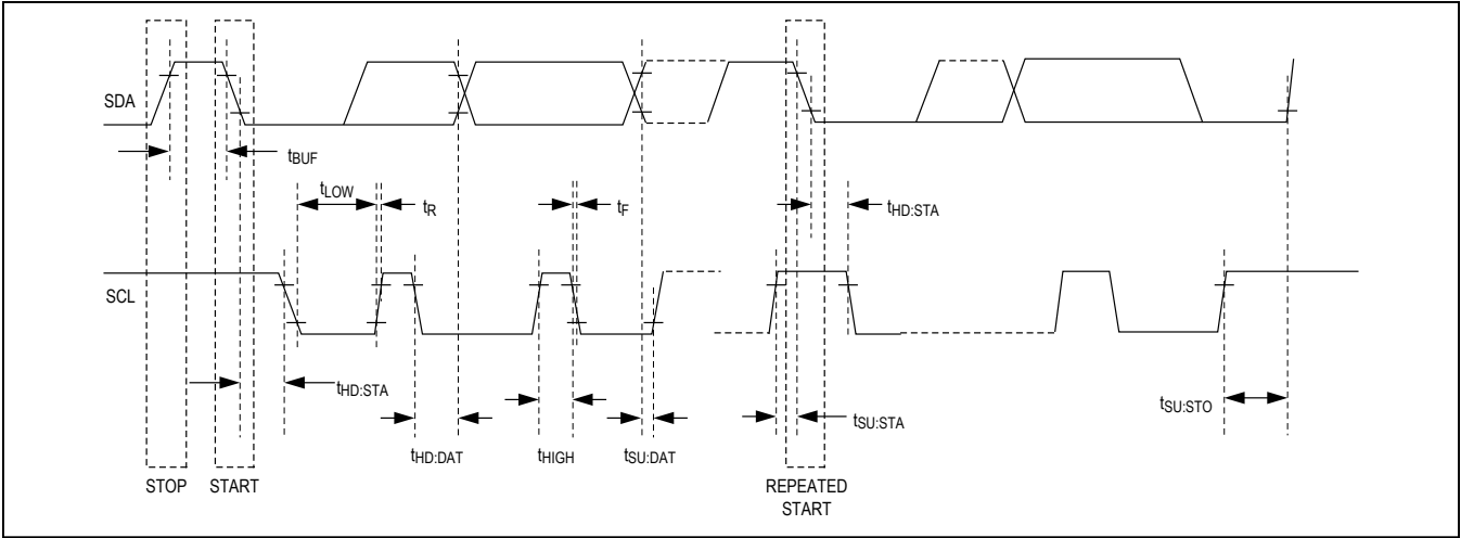
Figure 5. Timing Diagram
