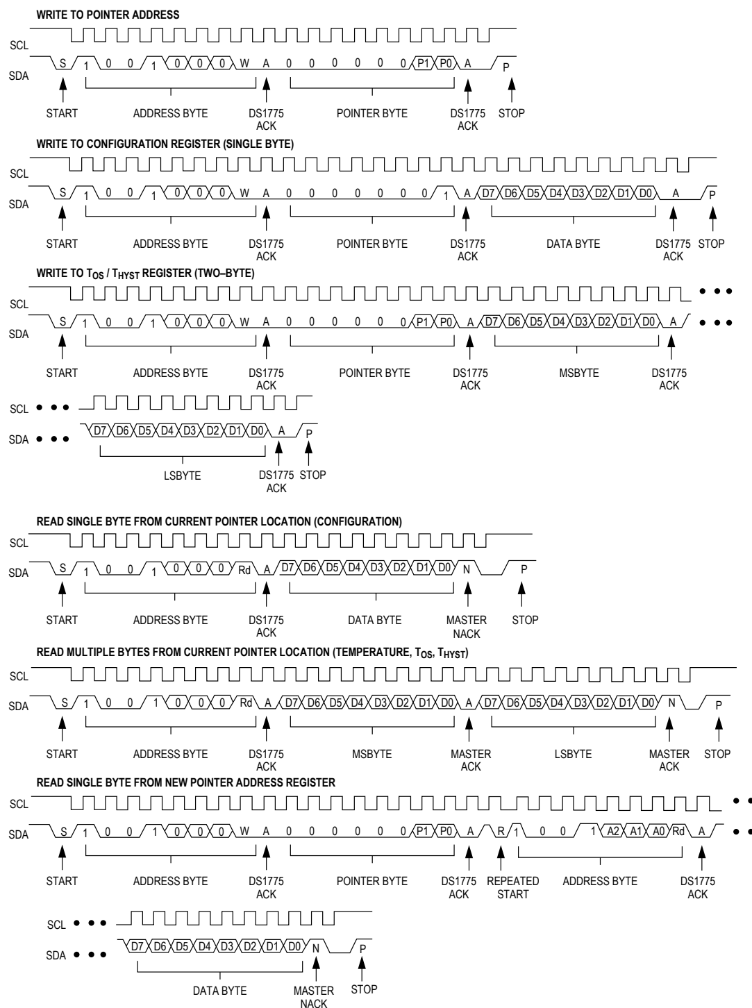
Figure 4. 2-Wire Serial Communication with DS1775
