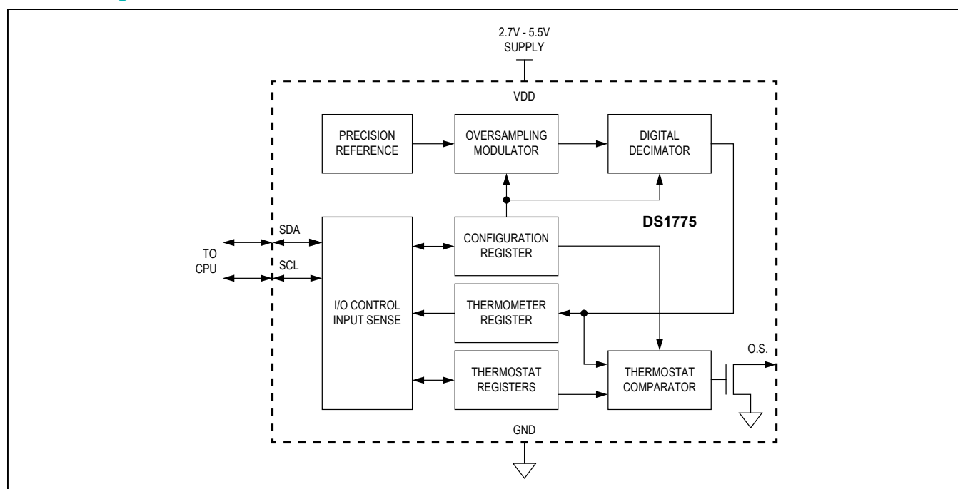
Figure 1. Block Diagram
