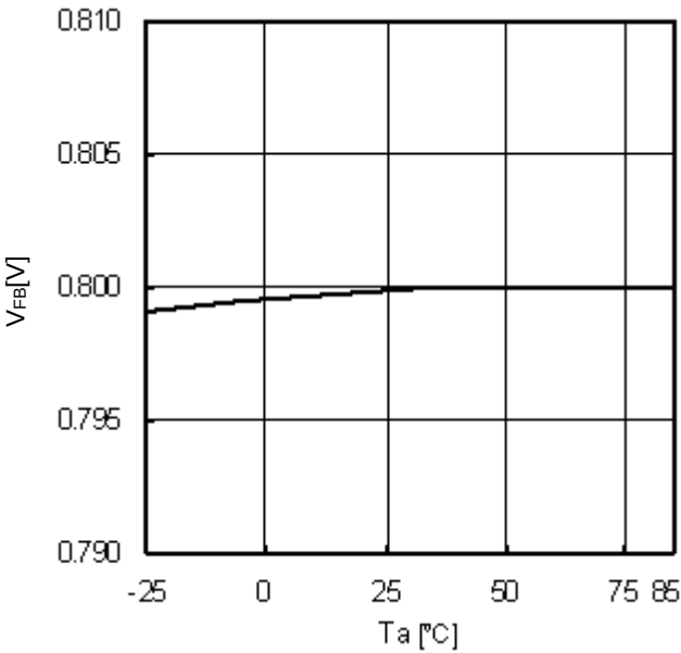
Fig.9 Ta-V FB
