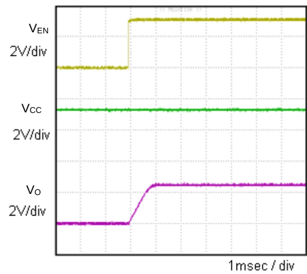
Fig.7 Input sequence2 Co=1.0μF
