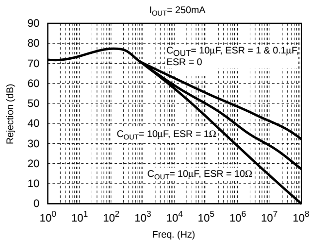
Ripple Rejection
