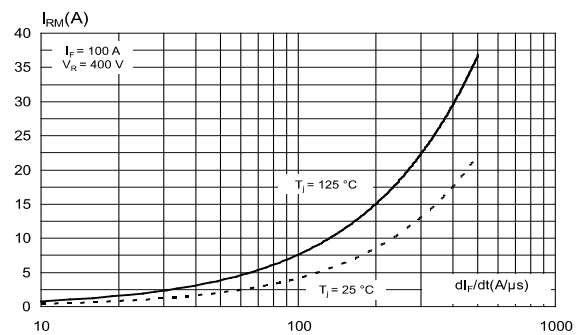
Figure 4: Peak reverse recovery current versus di/dt (typical values, per diode)
