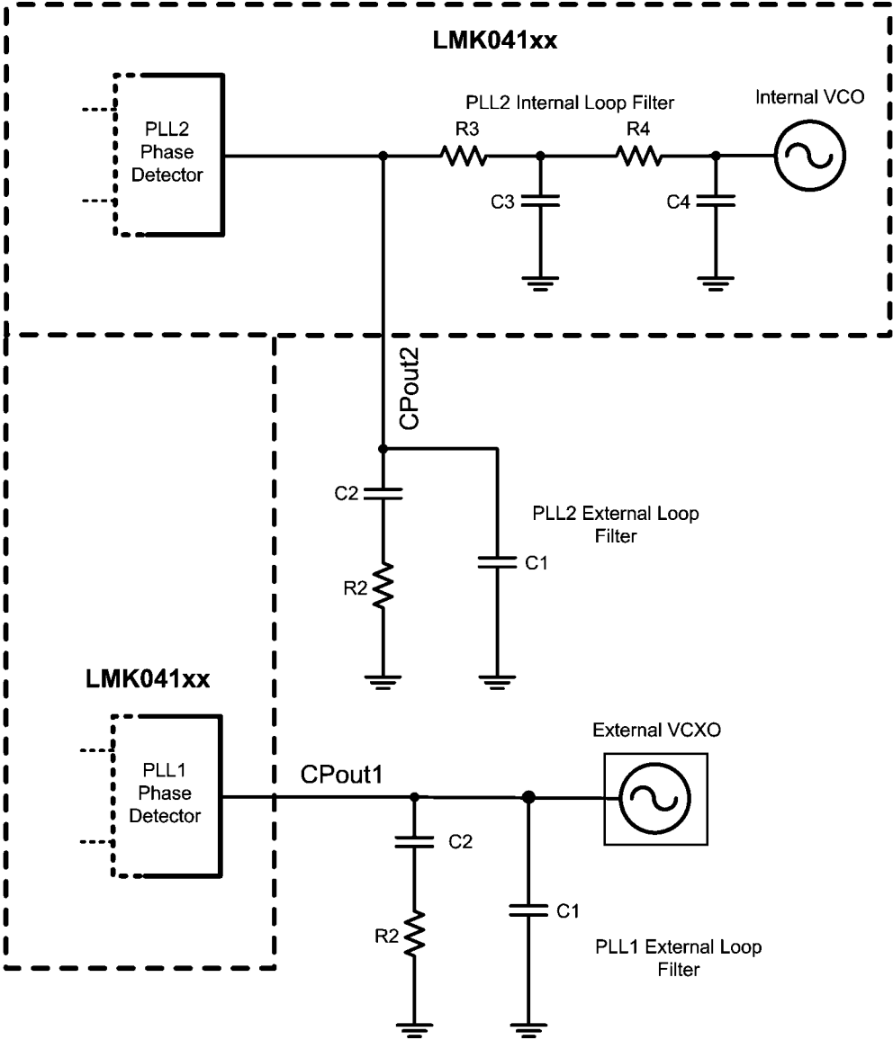
FIGURE 4. Loop Filter
