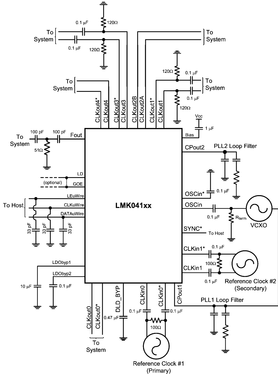
FIGURE 3. Typical Application
