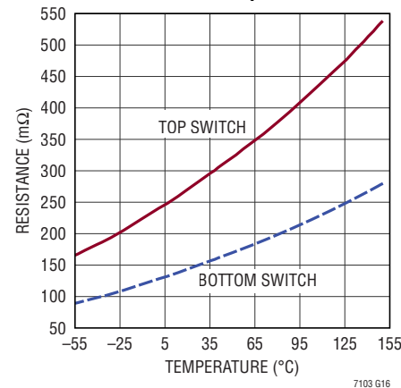
Top and Bottom Switch Resistance vs Temperature
