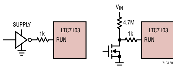
Figure 7. RUN Pin Interface to Logic
