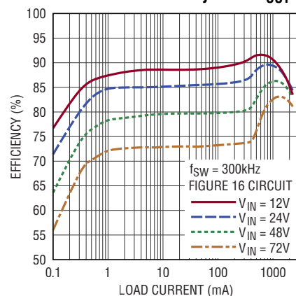
Burst Mode Efficiency at 3.3V OUT
