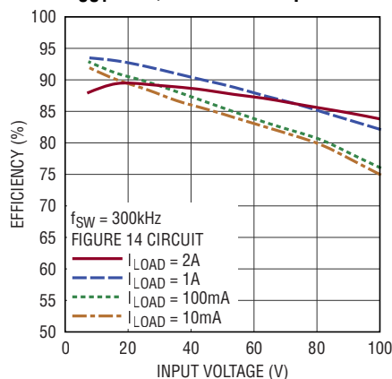
Efficiency vs Input Voltage V OUT = 5V, Burst Mode Operation
