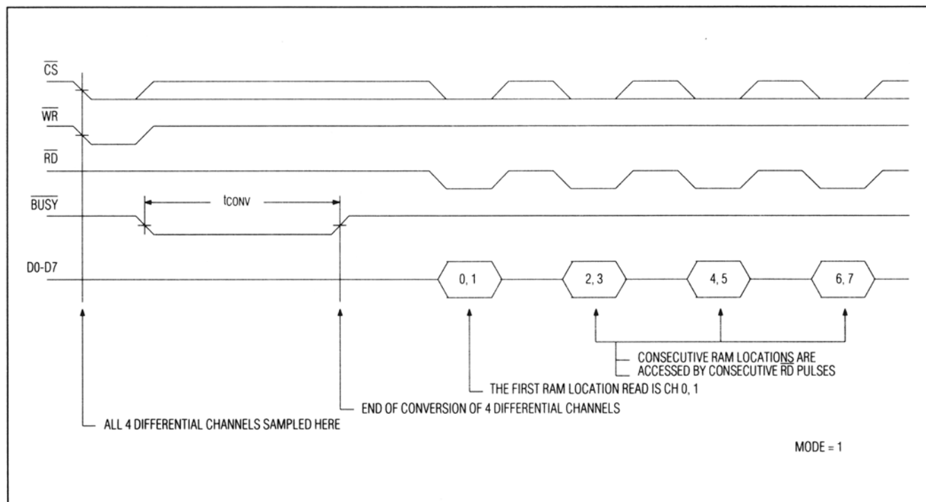
Figure 7b. Hard-Wired Mode Timing - Four Differential Conversions
