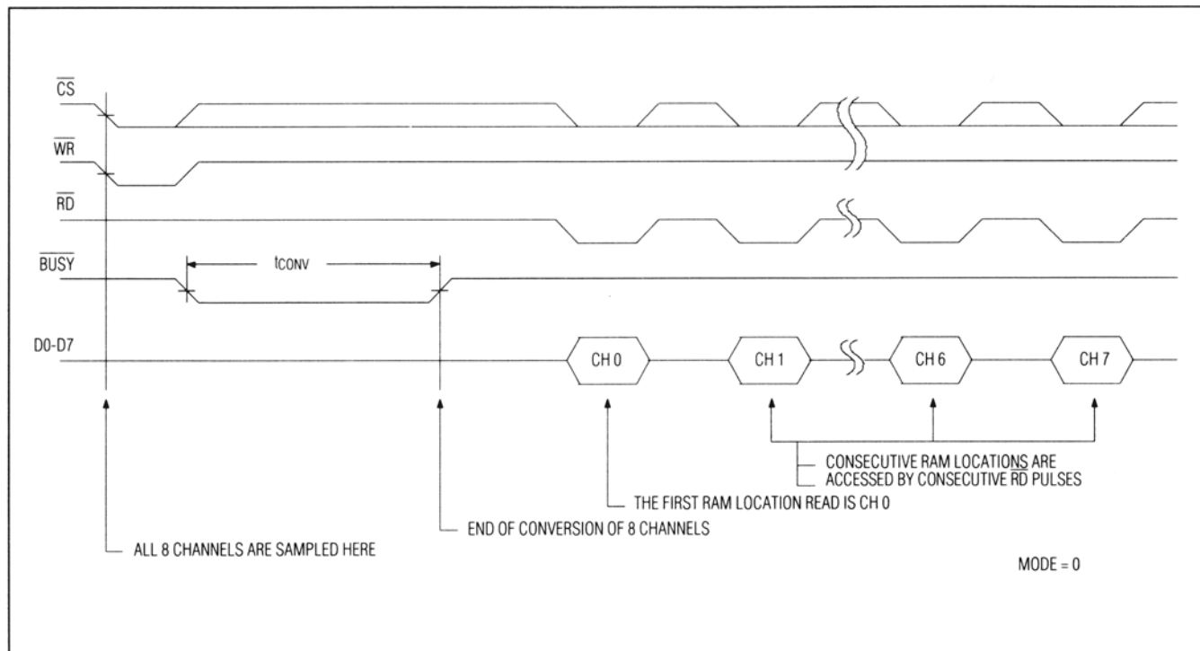
Figure 7a. Hard-Wired Mode Timing - Eight Single-Ended Conversions
