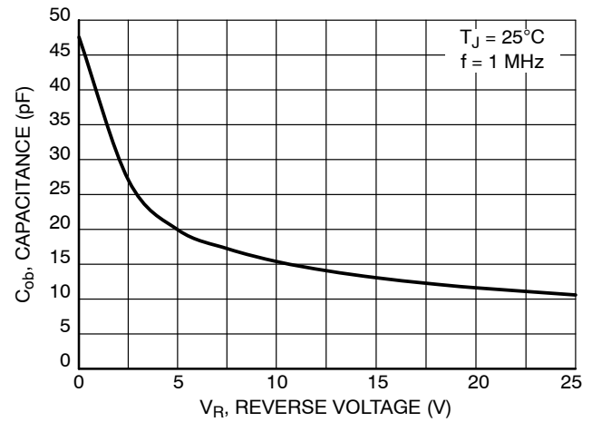
Figure 10. Output Capacitance
