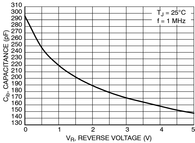
Figure 9. Input Capacitance
