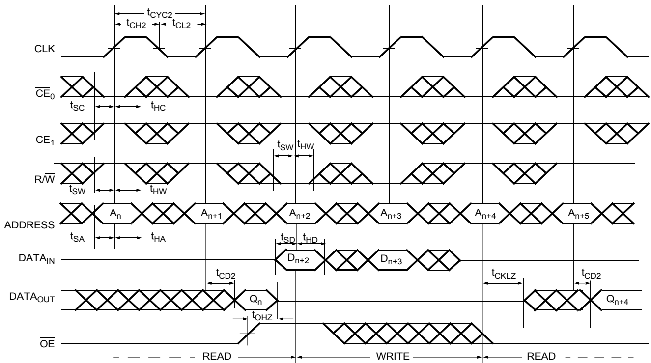
Figure 10. Pipelined Read-to-Write-to-Read ( \overline{OE} Controlled) [27, 28, 29, 30]
