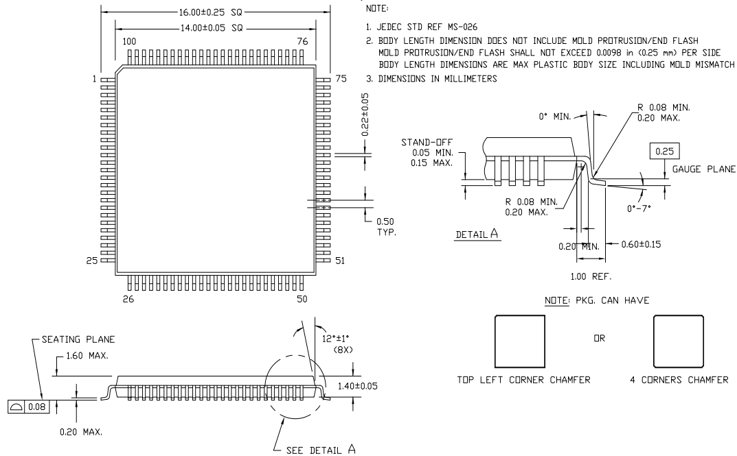
Figure 17. 100-Pin Thin Plastic Quad Flat Pack (TQFP), 51-85048
