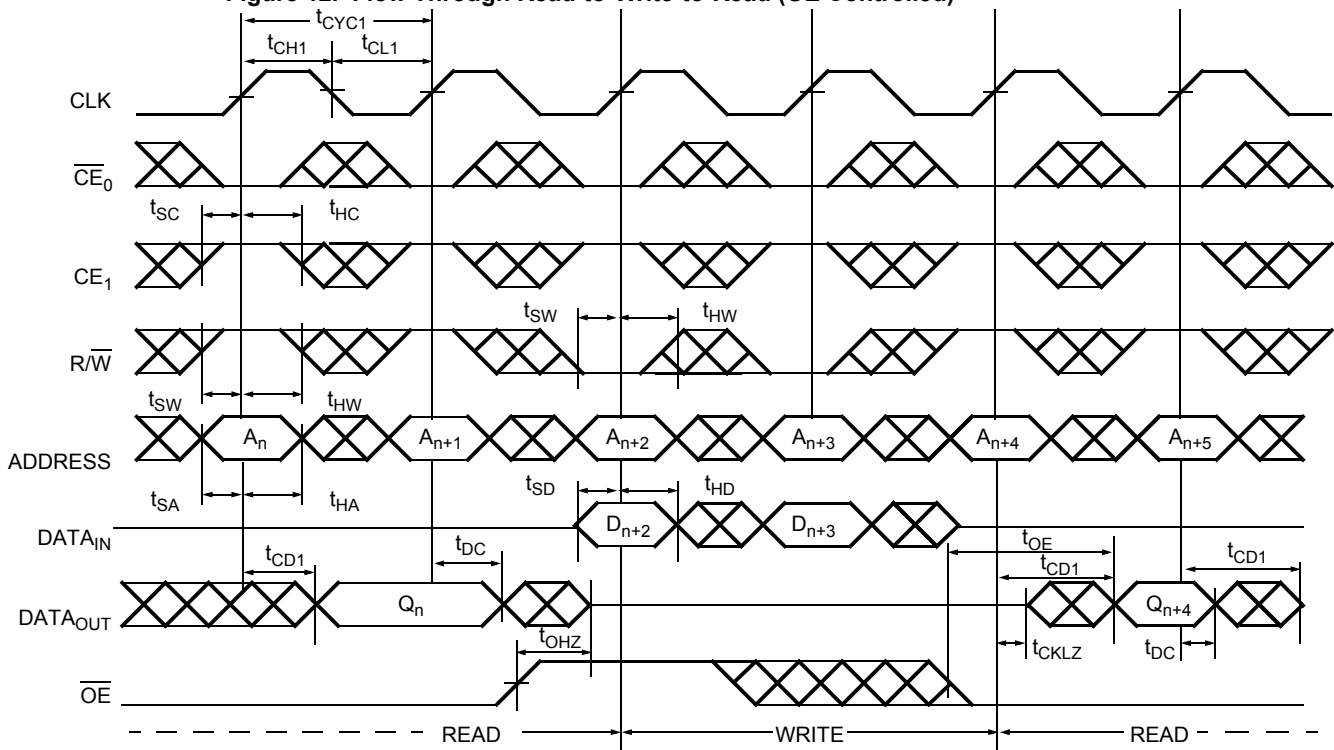
Figure 12. Flow Through Read-to-Write-to-Read ( \overline{OE} Controlled) [31, 32, 33, 34, 35]
