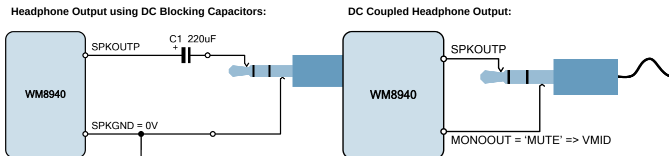
Figure 23 Recommended Headphone Output Configurations
