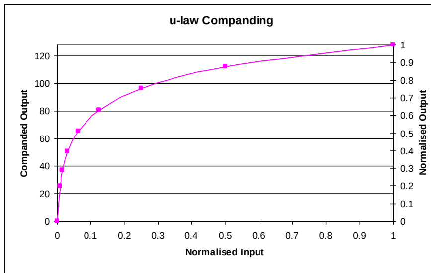
Figure 31 u-Law Companding
