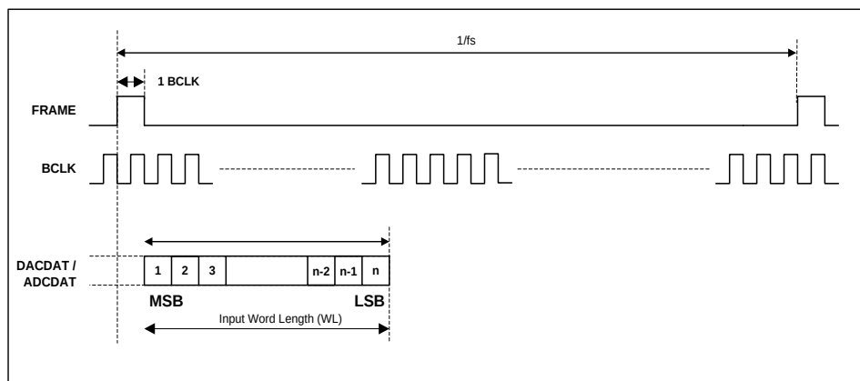
Figure 28 DSP/PCM Mode Audio Interface (Mode A, FRAMEP=0)
