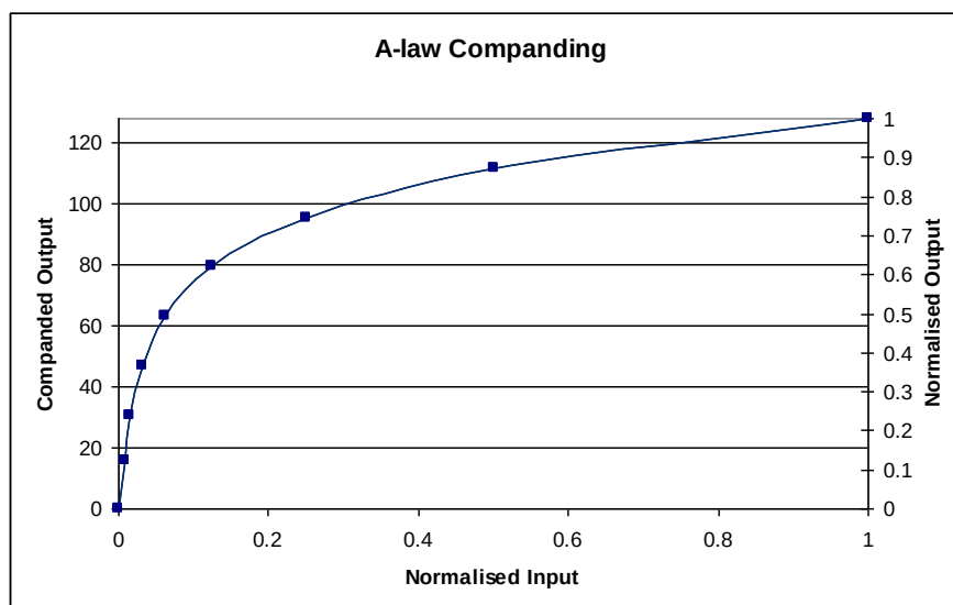
Figure 32 A-Law Companding
