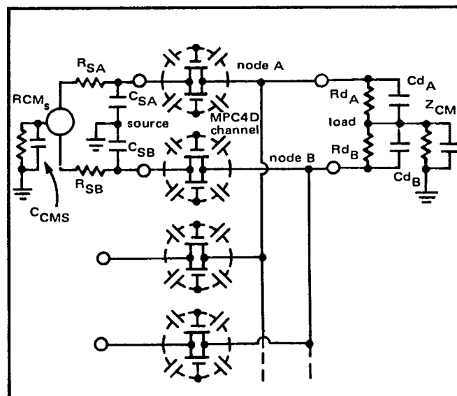
FIGURE 4: Settling & Common-Mode Effects – MPC4D.
