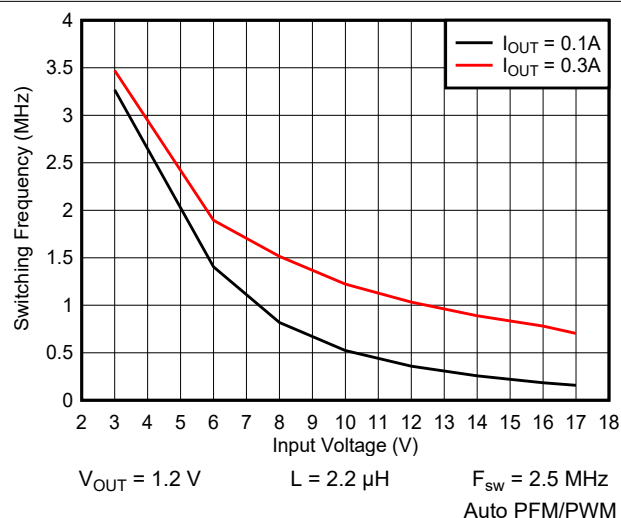
Figure 9-40. Switching Frequency vs Input Voltage
