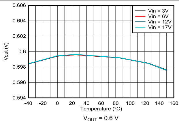
Figure 7-8. Output Voltage Accuracy – VSET Selected
