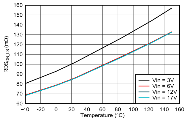
Figure 7-12. Low-Side R_{DS_{ON}} vs Temperature
