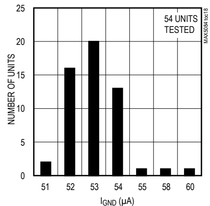
GROUND CURRENT DISTRIBUTION (T A = +125°C)
