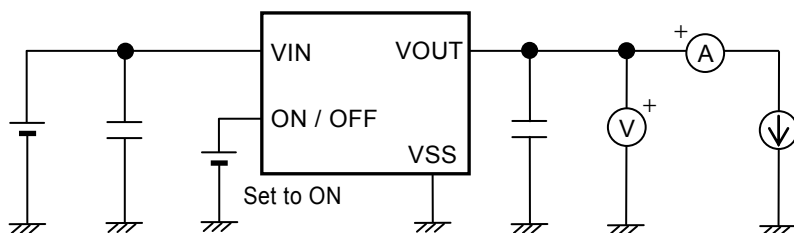
Figure 10 Test Circuit 1
