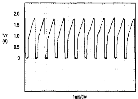
INPUT CURRENT (VCC OUTPUT SHORTED)
