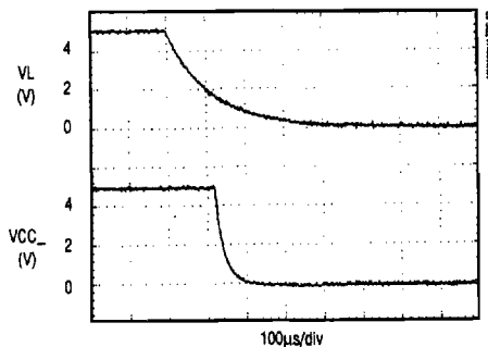
VCC_ SHUTDOWN RESPONSE
