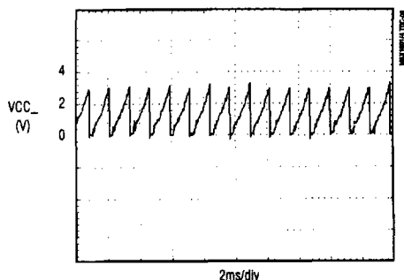
VCC_ CURRENT LIMITING
