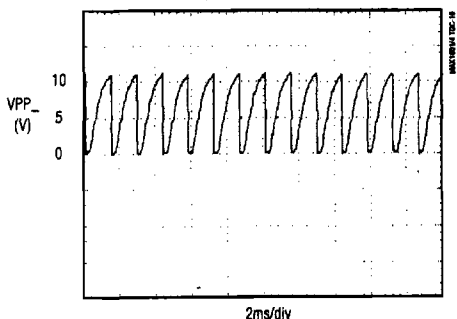
VPP_ CURRENT LIMITING
