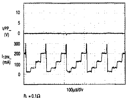
INPUT CURRENT (VPP OUTPUT SHORTED)
