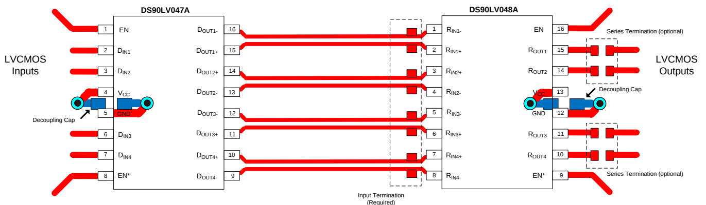
Figure 23. Layout Recommendation
