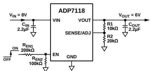
Figure 47. Typical EN Pin Voltage Divider
