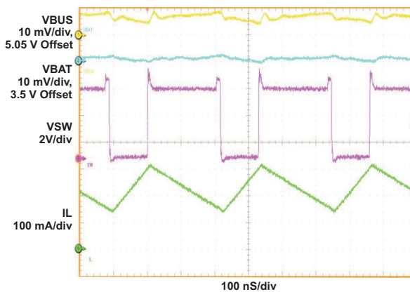
BOOST WAVEFORM (PWM MODE)
