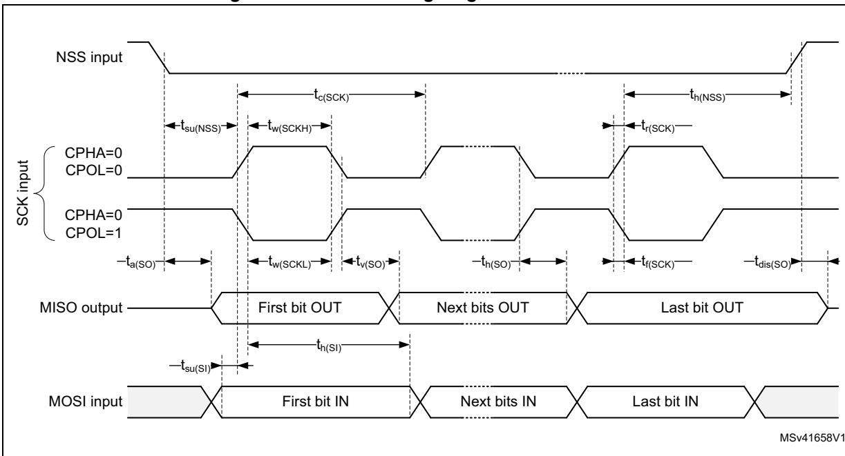
Figure 52. USART timing diagram in Slave mode
