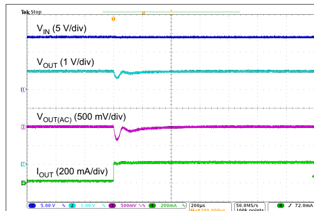
Figure 5-19. Load Transient
