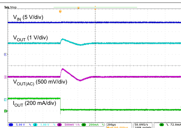
Figure 5-20. Load Transient
