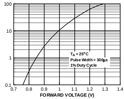
Figure 2. Forward Characteristics
