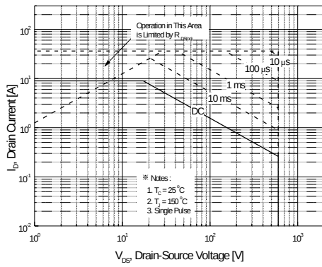
Figure 9-1. Maximum Safe Operating Area for SSP10N60B
