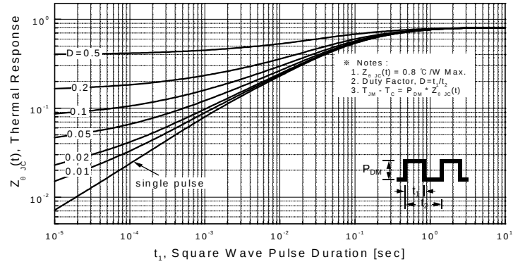
Figure 11-1. Transient Thermal Response Curve for SSP10N60B
