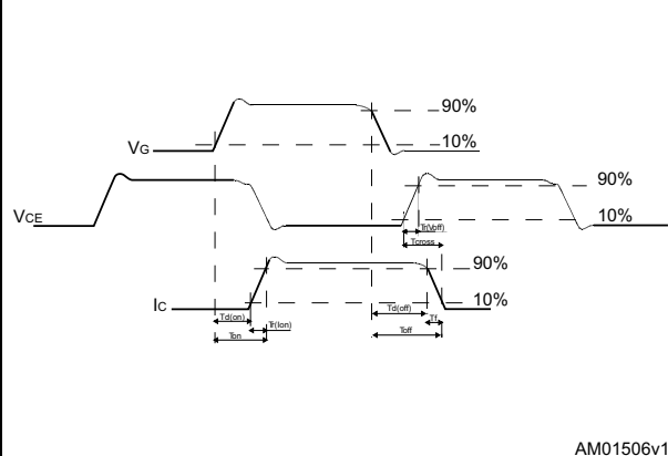
Figure 29. Switching waveform
