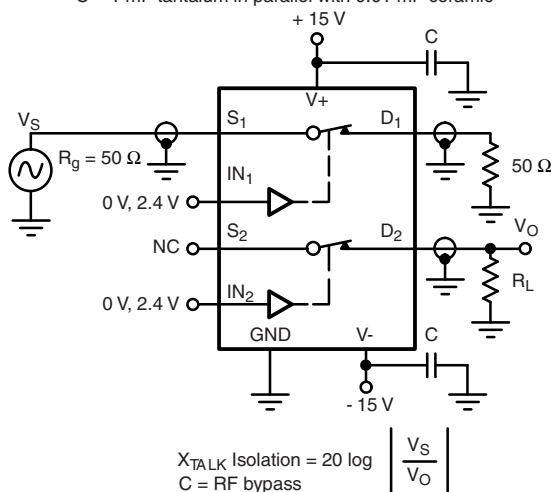
Fig. 4 - Crosstalk
