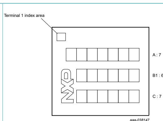
Figure 3. PN7150 package marking HVQFN40 (top view) 3 lines
