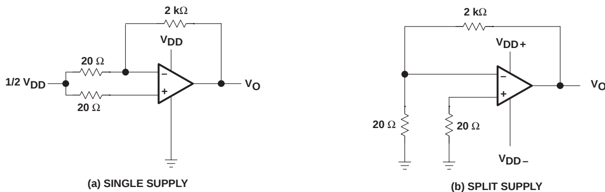
Figure 27. Noise-Test Circuit
