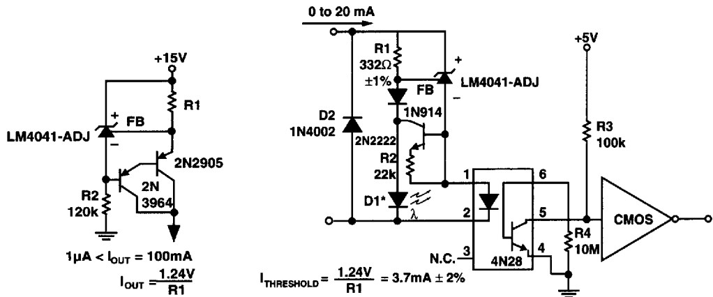
Figure 10. Current Source
