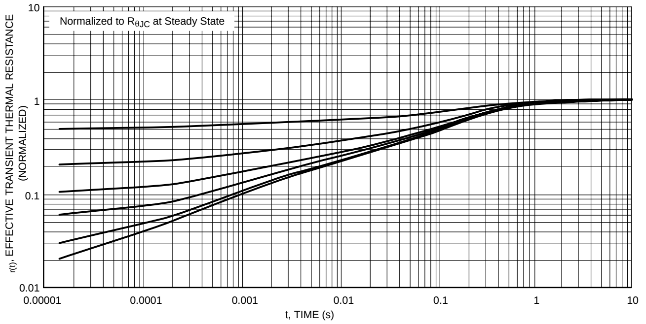
Figure 12. Thermal Response
