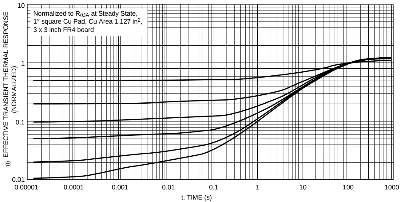
Figure 13. Thermal Response
