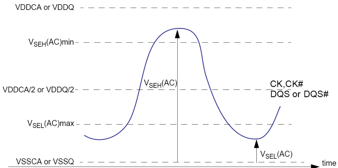
Figure 7.5 — Single-ended requirement for differential signals.
