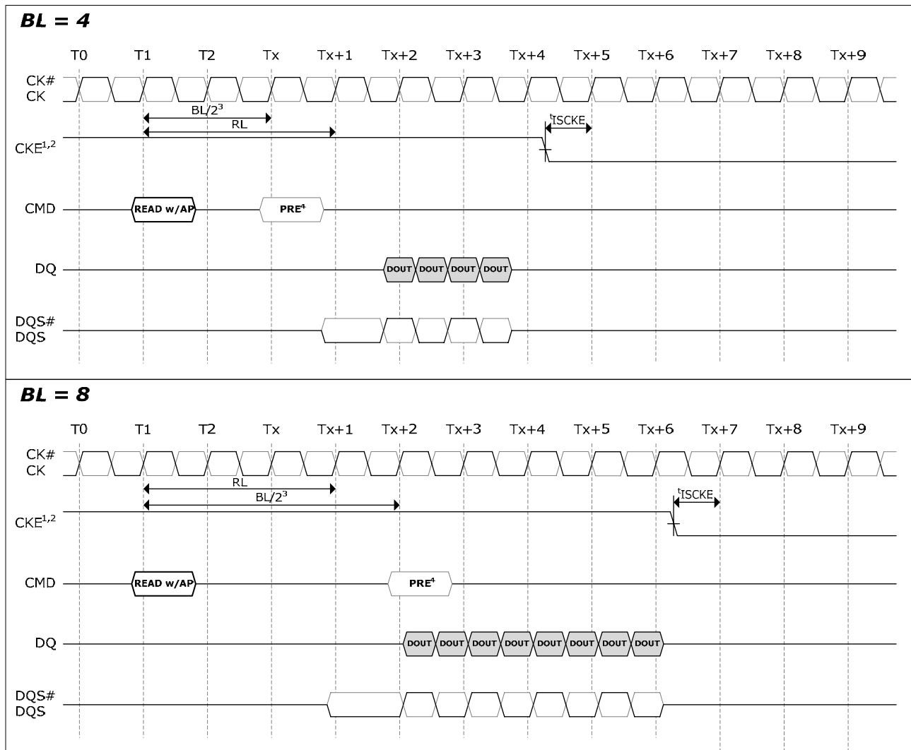
Figure 4.48 — LPDDR2 SDRAM Read with autprecharge to power-down entry
