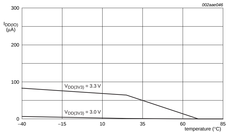
Fig 7. I/O maximum supply current I_{DD(IO)} versus temperature in Deep power-down mode
