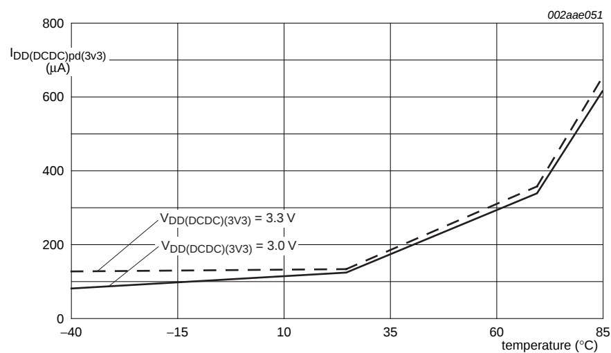
Fig 6. Total DC-to-DC converter supply current I_{DD(DCDC)pd(3V3)} at different temperatures in Power-down mode
