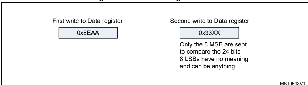
Figure 267. Transmitting 0x8EAA33
