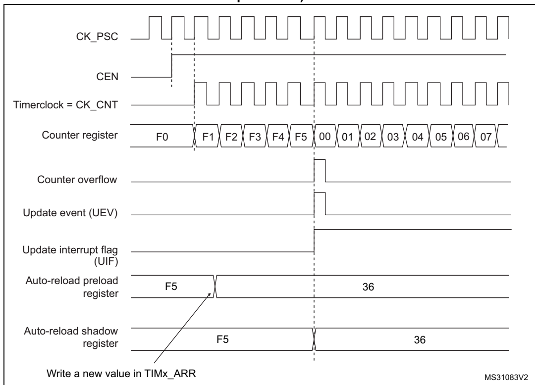
Figure 131. Counter timing diagram, update event when ARPE=1 (TIMx_ARR preloaded)
