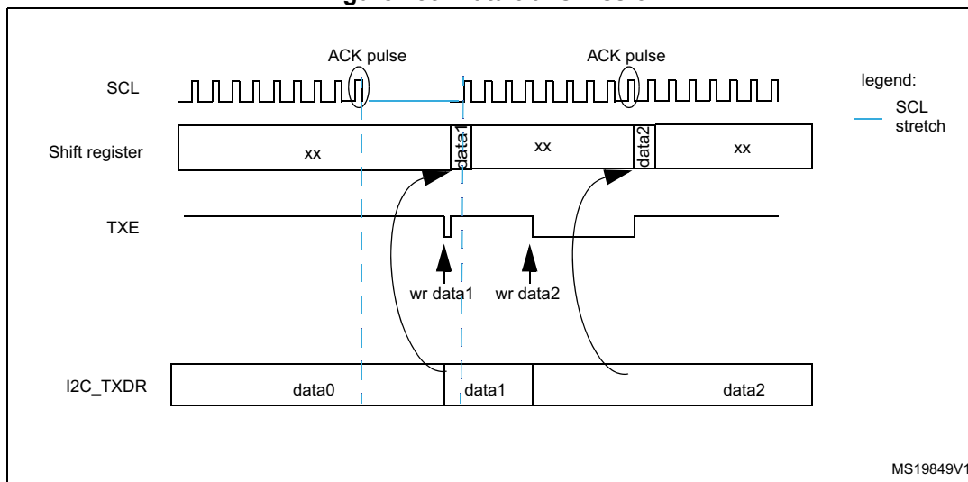
Figure 188. Data transmission
