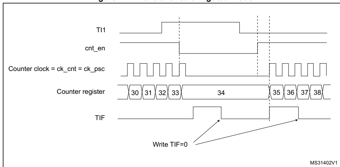
Figure 114. Control circuit in gated mode
