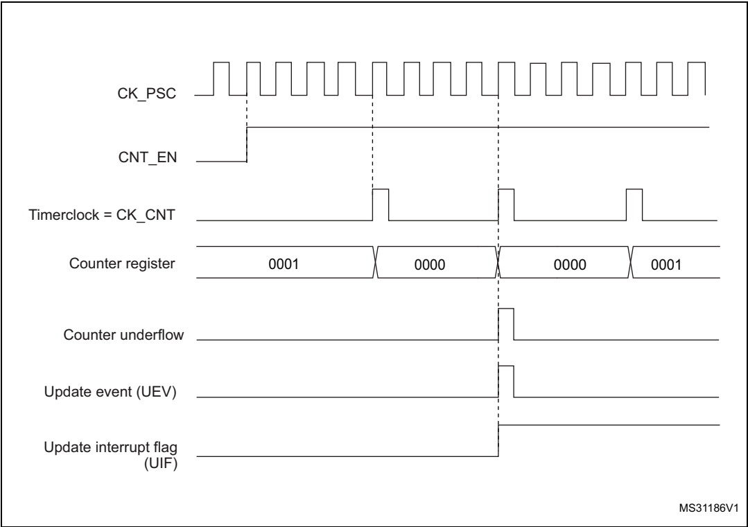
Figure 134. Counter timing diagram, internal clock divided by 4
