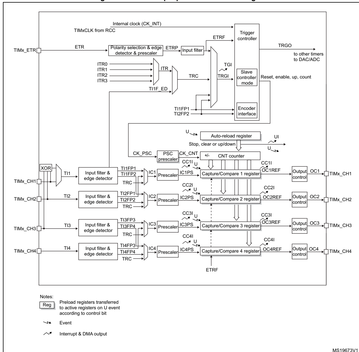
Figure 77. General-purpose timer block diagram
