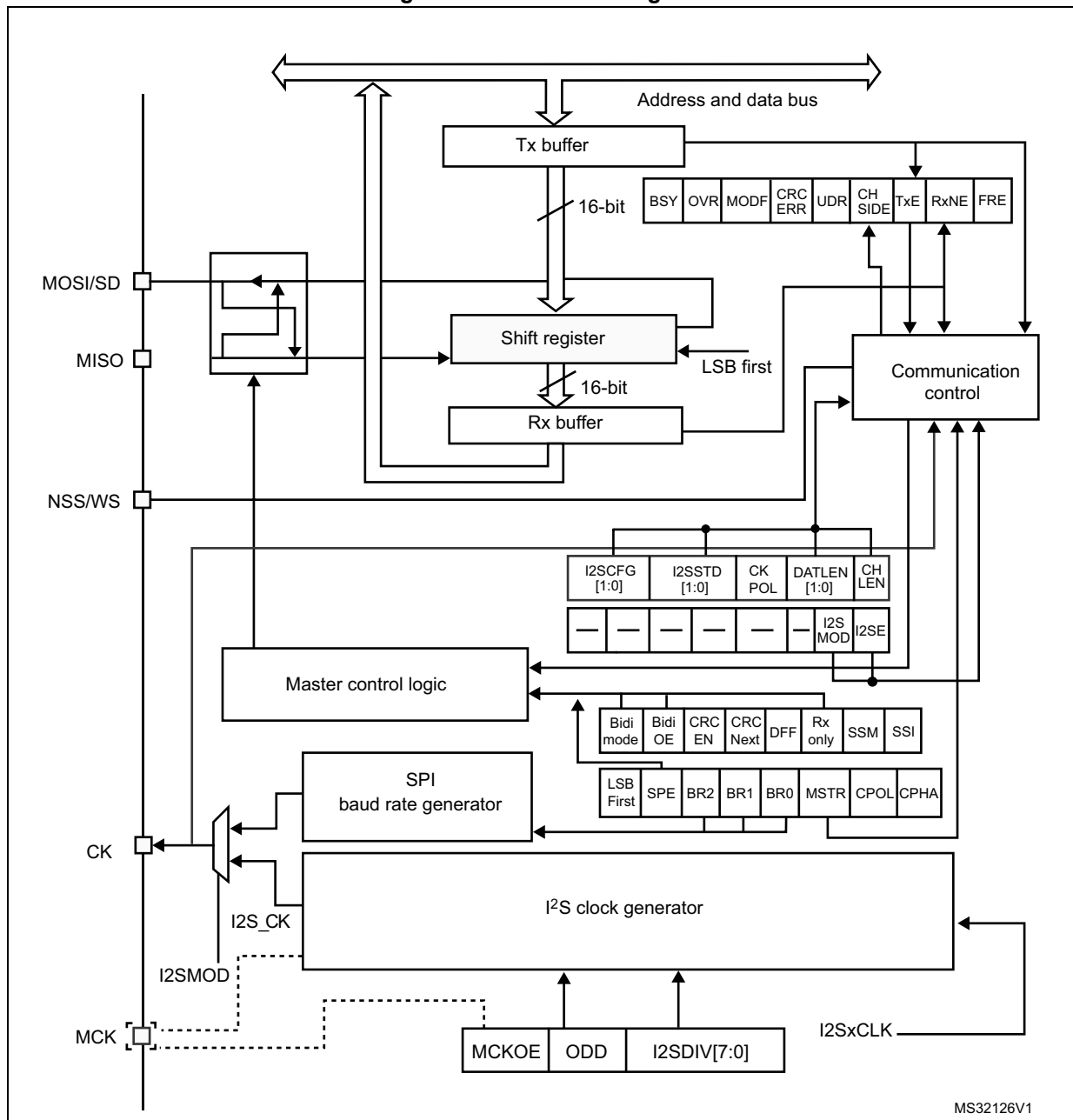
Figure 263. I 2 S block diagram
