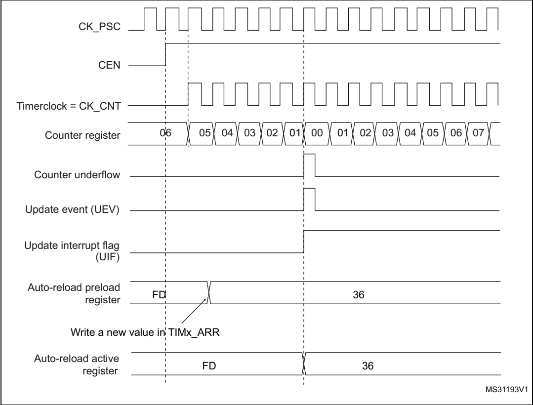
Figure 95. Counter timing diagram, Update event with ARPE=1 (counter underflow)
