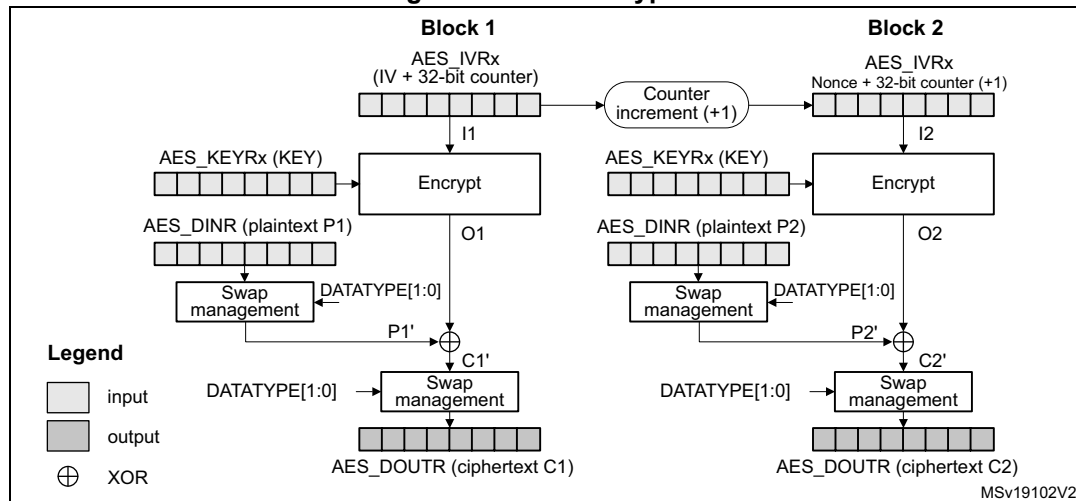
Figure 71. CTR encryption
