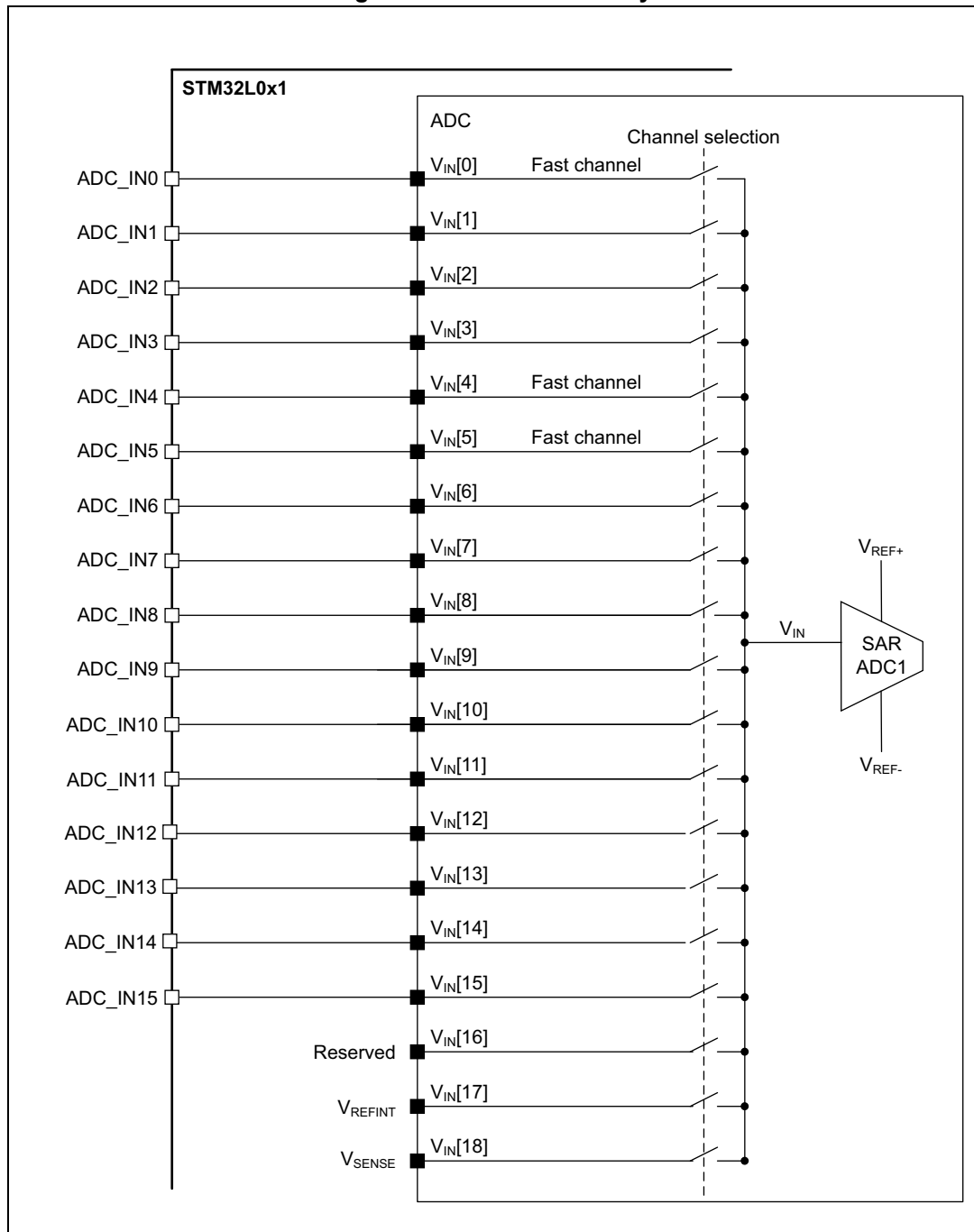
Figure 34. ADC connectivity
