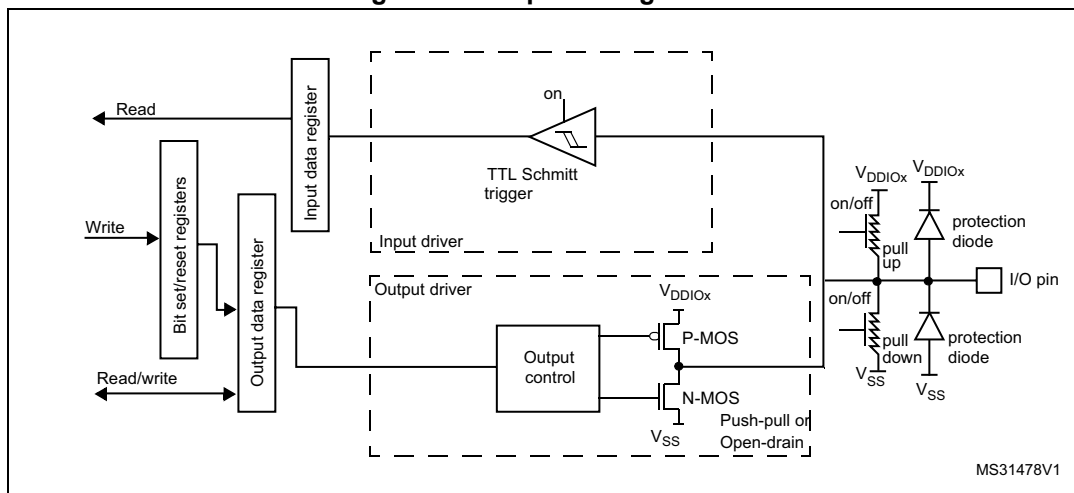
Figure 22. Output configuration
