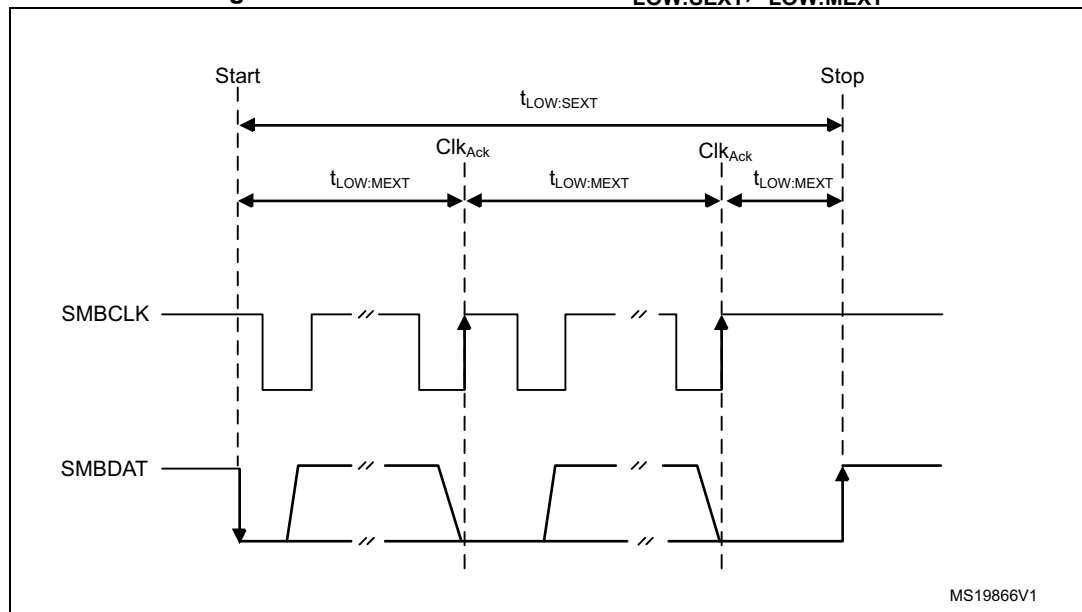
Figure 206. Timeout intervals for t_{\text{LOW:SEXT}} , t_{\text{LOW:MEXT}}
