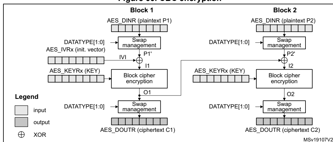
Figure 66. CBC encryption
