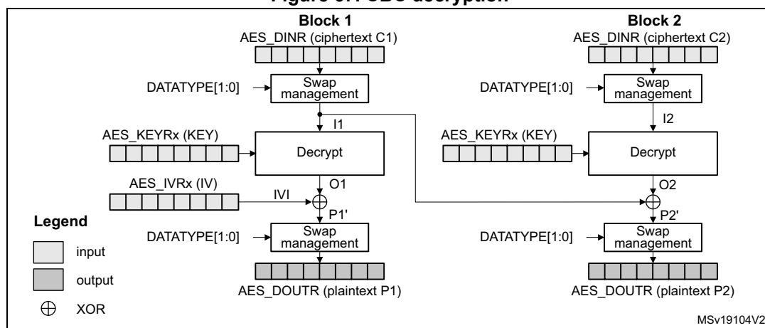
Figure 67. CBC decryption
