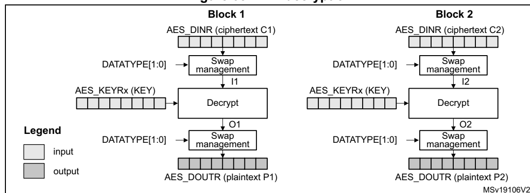
Figure 65. ECB decryption
