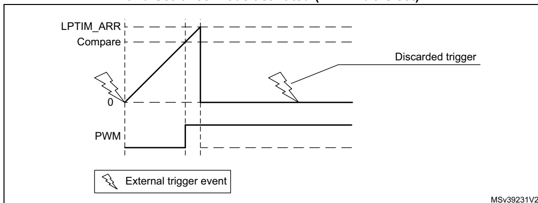
Figure 174. LPTIM output waveform, Single counting mode configuration and Set-once mode activated (WAVE bit is set)
