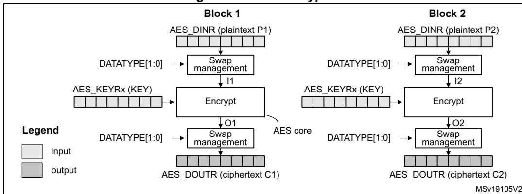
Figure 64. ECB encryption
