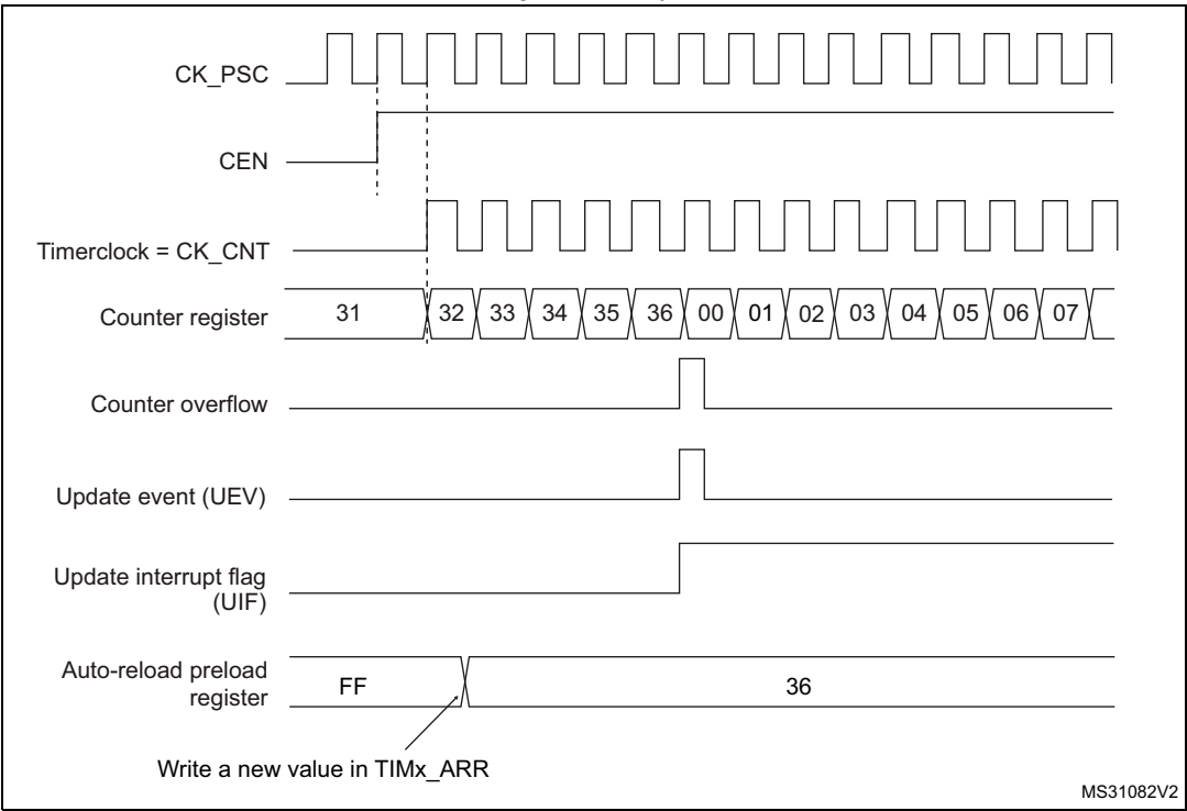
Figure 130. Counter timing diagram, update event when ARPE=0 (TIMx_ARR not preloaded)
