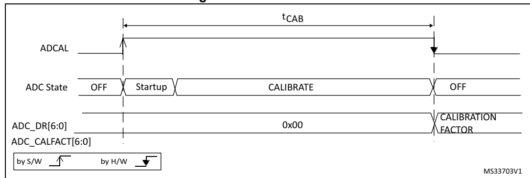
Figure 30. ADC calibration
