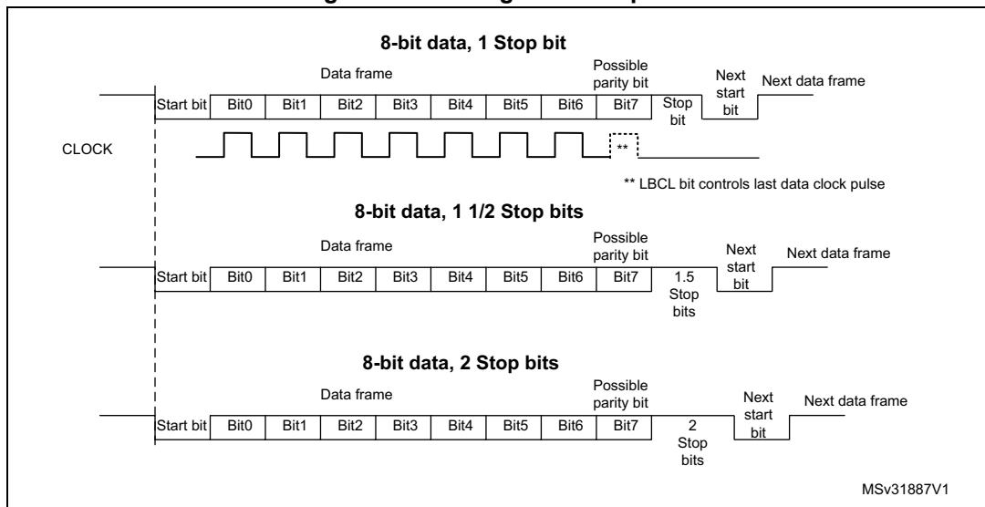
Figure 215. Configurable stop bits
