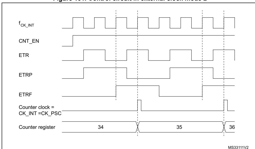
Figure 101. Control circuit in external clock mode 2
