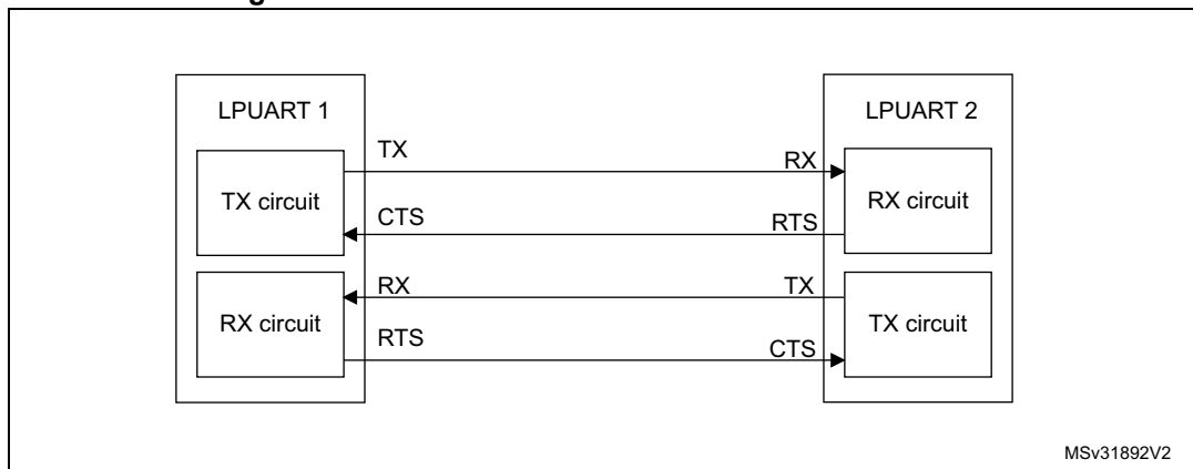
Figure 246. Hardware flow control between 2 LPUARTs
