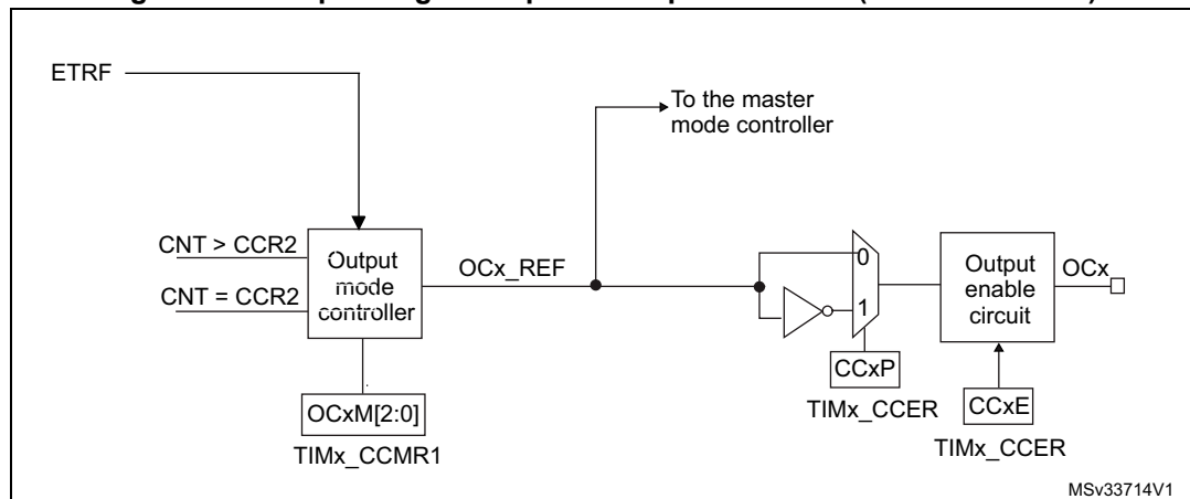
Figure 149. Output stage of capture/compare channel (channel 1 and 2)
