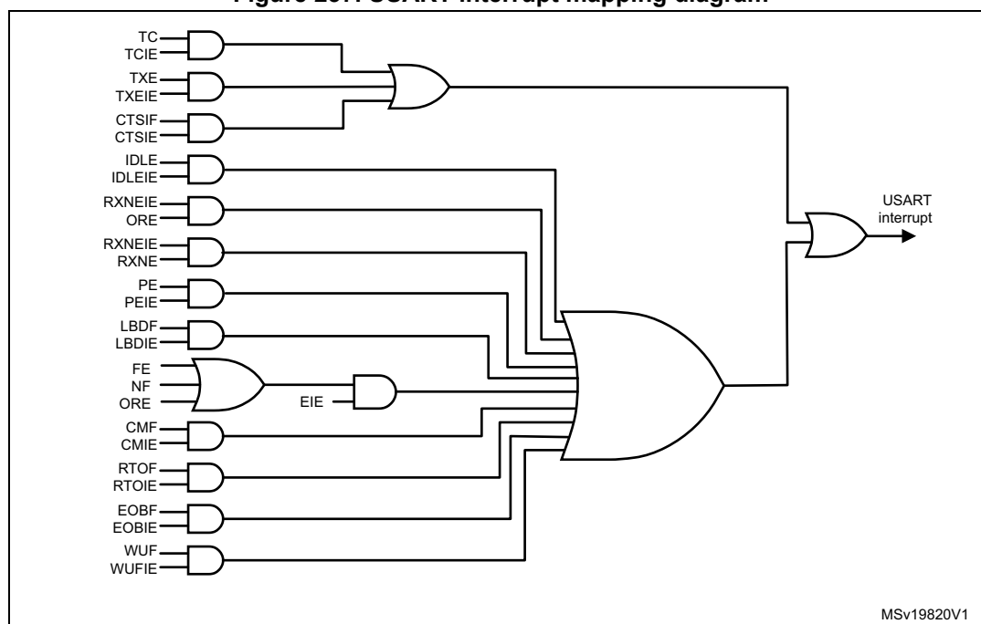
Figure 237. USART interrupt mapping diagram
