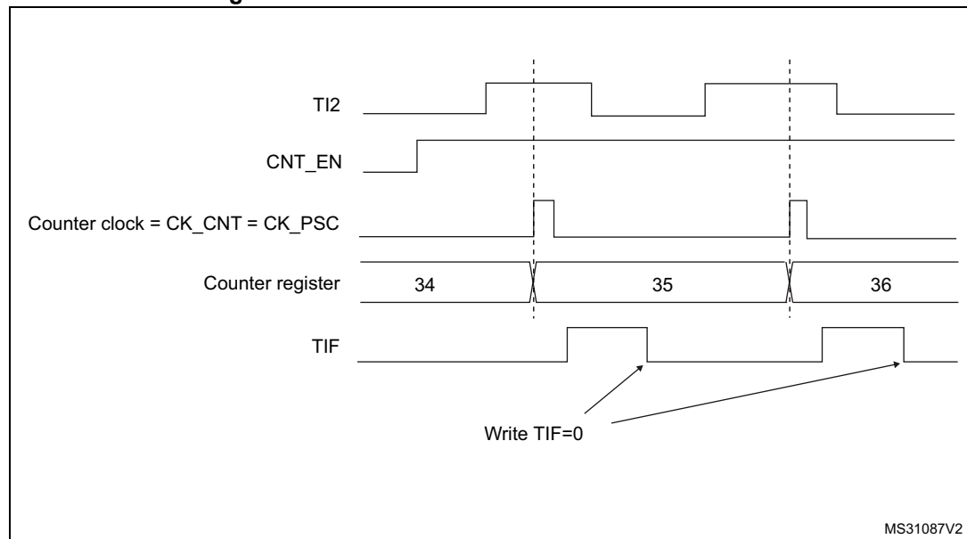
Figure 99. Control circuit in external clock mode 1
