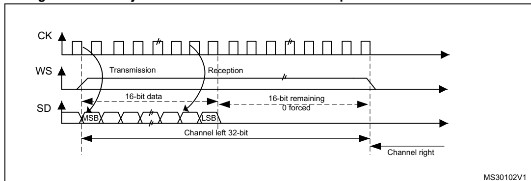
Figure 273. MSB justified 16-bit extended to 32-bit packet frame with CPOL = 0
