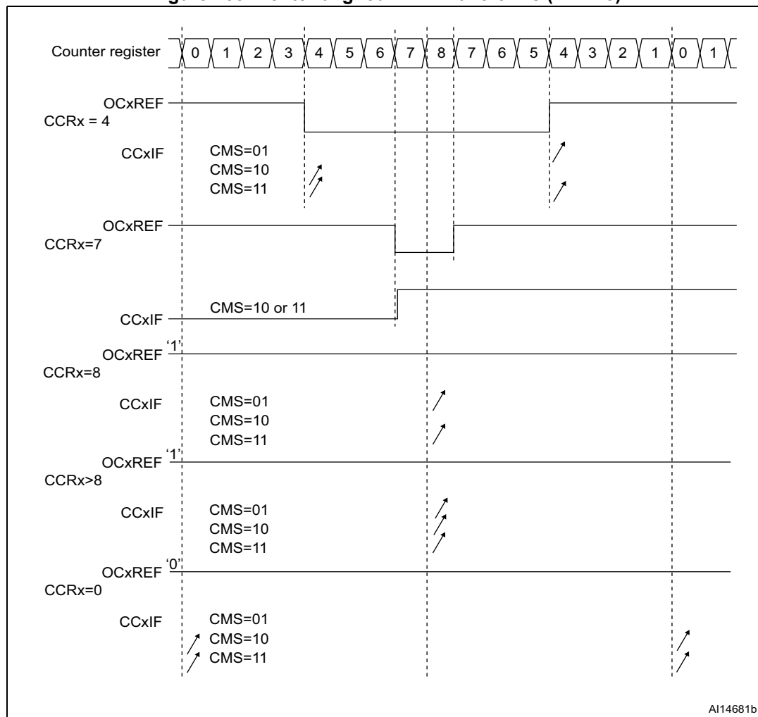
Figure 153. Center-aligned PWM waveforms (ARR=8)
