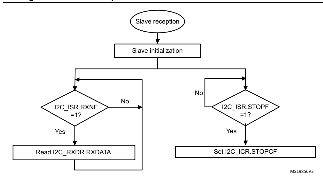
Figure 194. Transfer sequence flow for slave receiver with NOSTRETCH = 1
