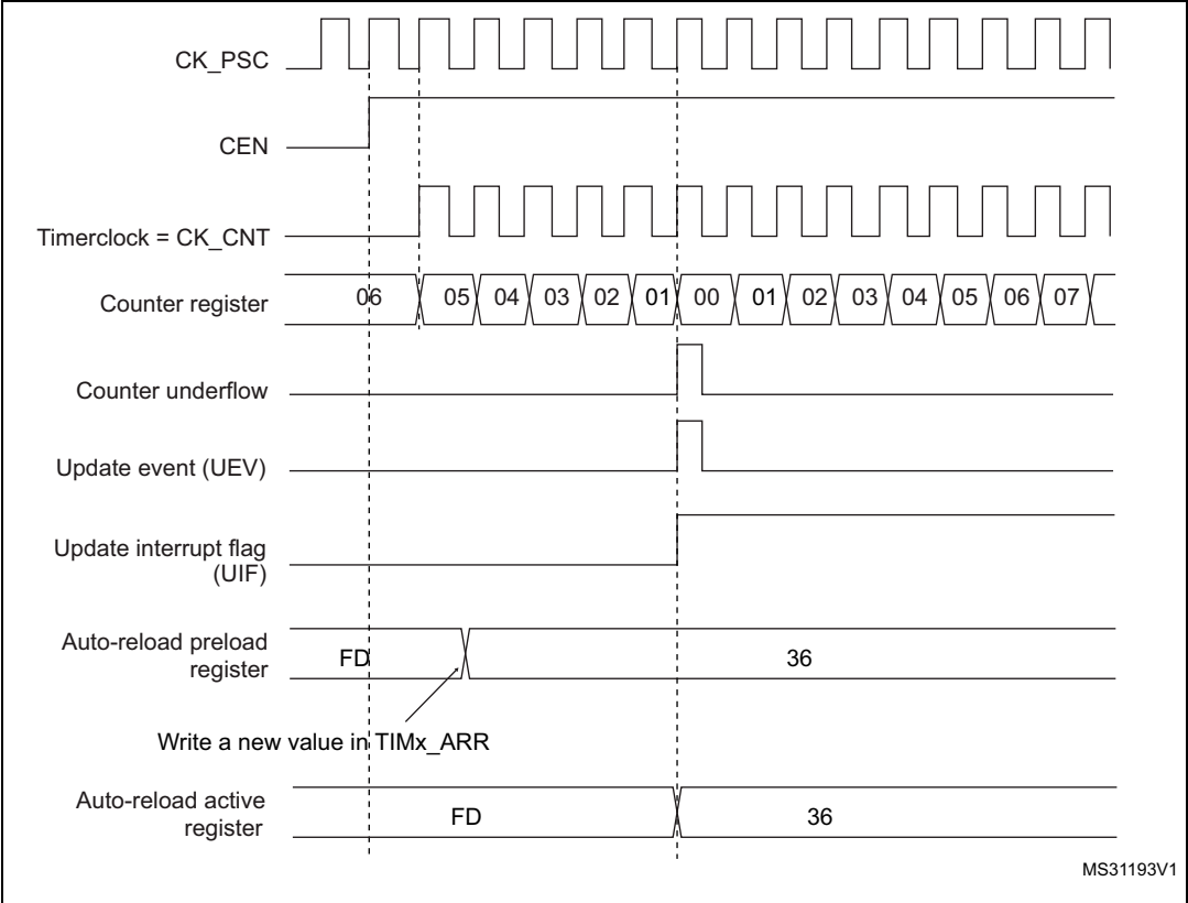
Figure 140. Counter timing diagram, Update event with ARPE=1 (counter underflow)
