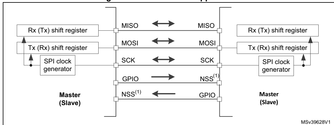
Figure 255. Multi-master application
