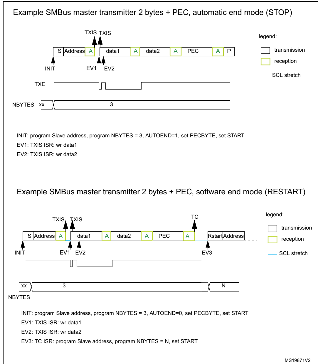
Figure 211. Bus transfer diagrams for SMBus master transmitter
