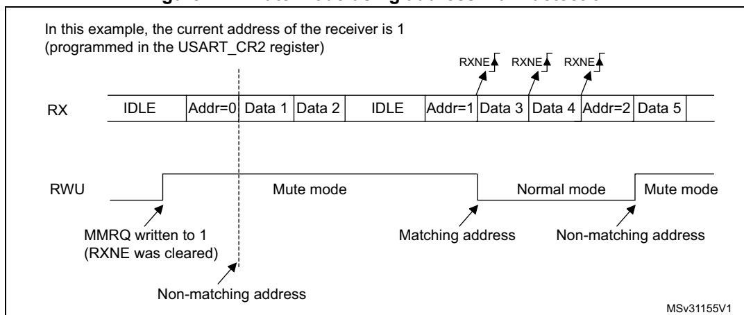
Figure 221. Mute mode using address mark detection
