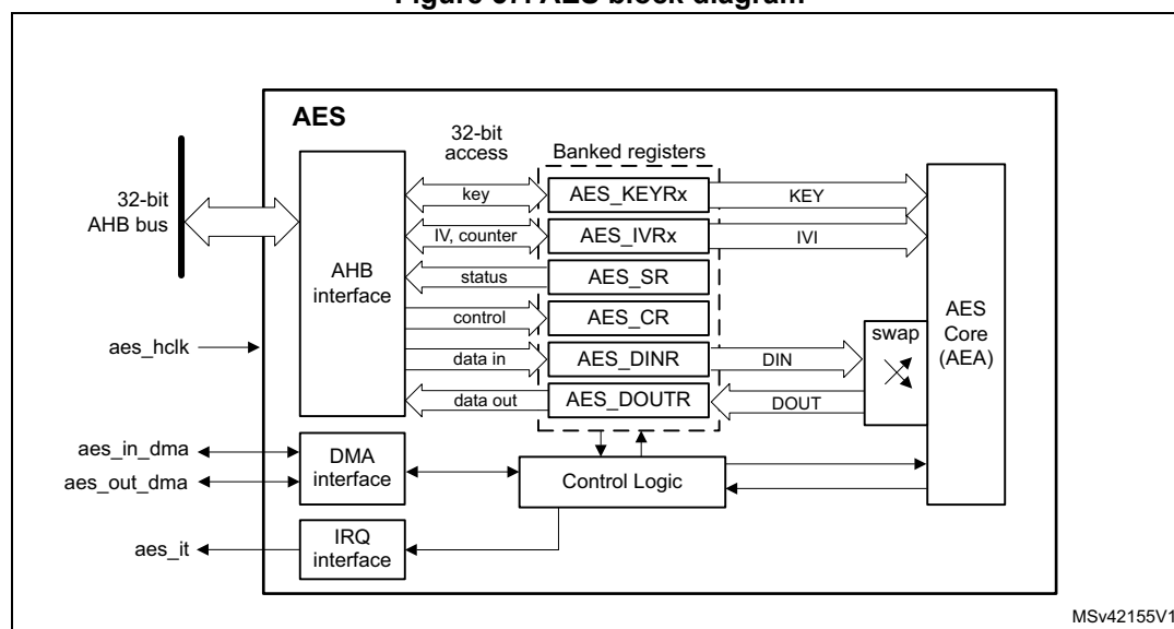
Figure 57. AES block diagram
