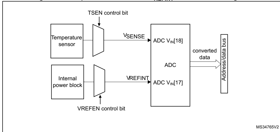
Figure 55. Temperature sensor and V_{\text{REFINT}} channel block diagram
