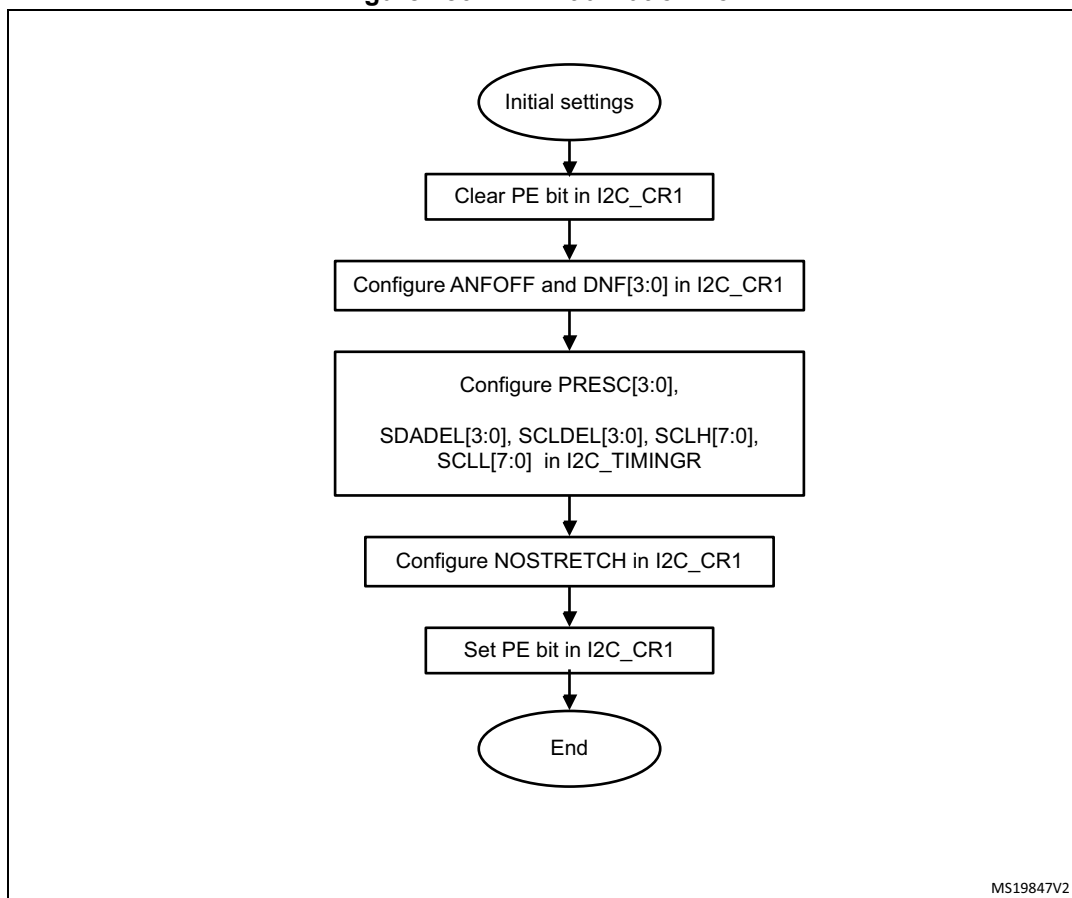
Figure 186. I2C initialization flow
