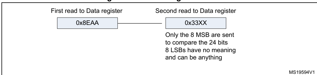
Figure 268. Receiving 0x8EAA33
