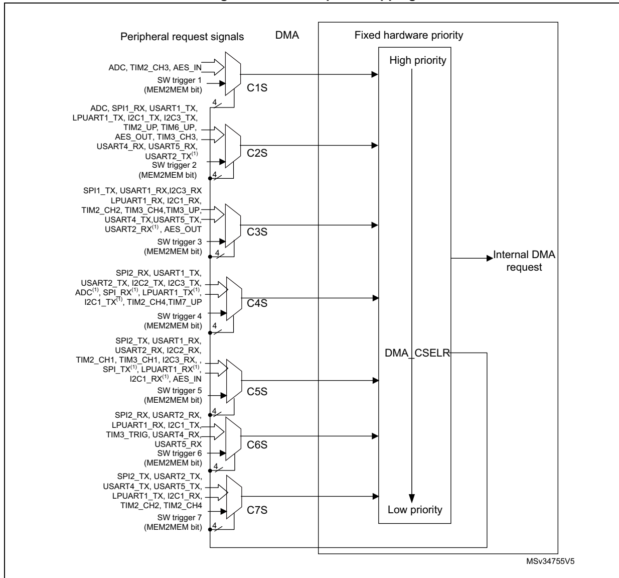
Figure 25. DMA request mapping
