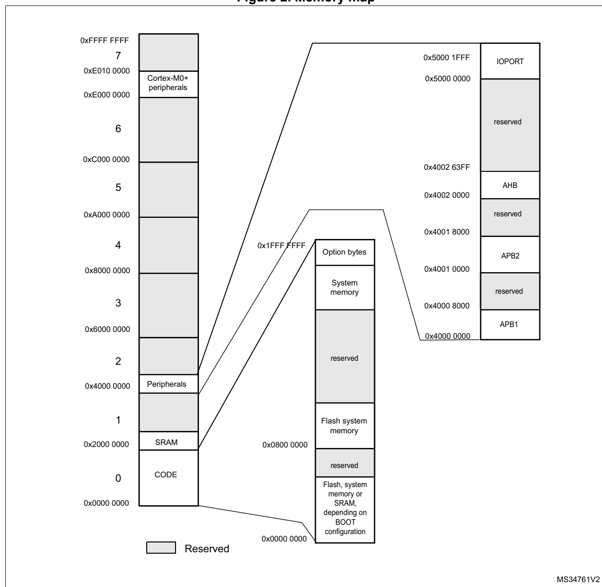
Figure 2. Memory map
